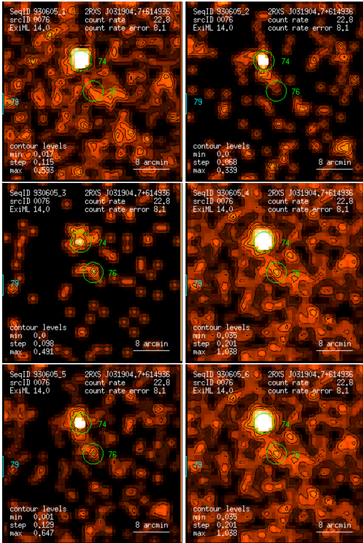
Figure 76: RASS 930605: detection 0076: band rate images, Gaussian filter: (1) PSPC channels 11 – 41, (2) 52 – 90, (3) 91 – 201, (4) 11 – 235, (5) 52 – 201, (6) 11 – 201. Broad band rates in counts/ks. Band rate contour levels in counts/ks/arcmin 2 .
