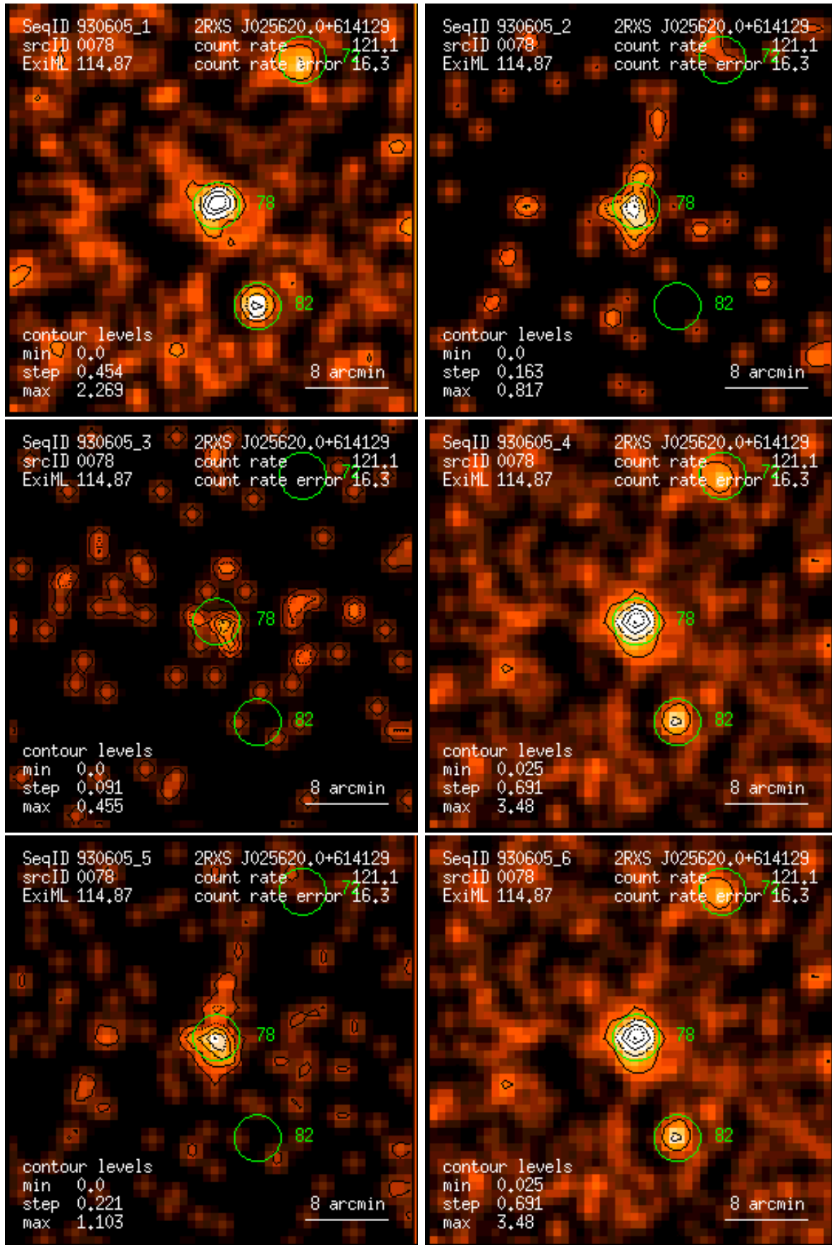
Figure 78: RASS 930605: detection 0078: band rate images, Gaussian filter: (1) PSPC channels 11 – 41, (2) 52 – 90, (3) 91 – 201, (4) 11 – 235, (5) 52 – 201, (6) 11 – 201. Broad band rates in counts/ks. Band rate contour levels in counts/ks/arcmin 2 .
