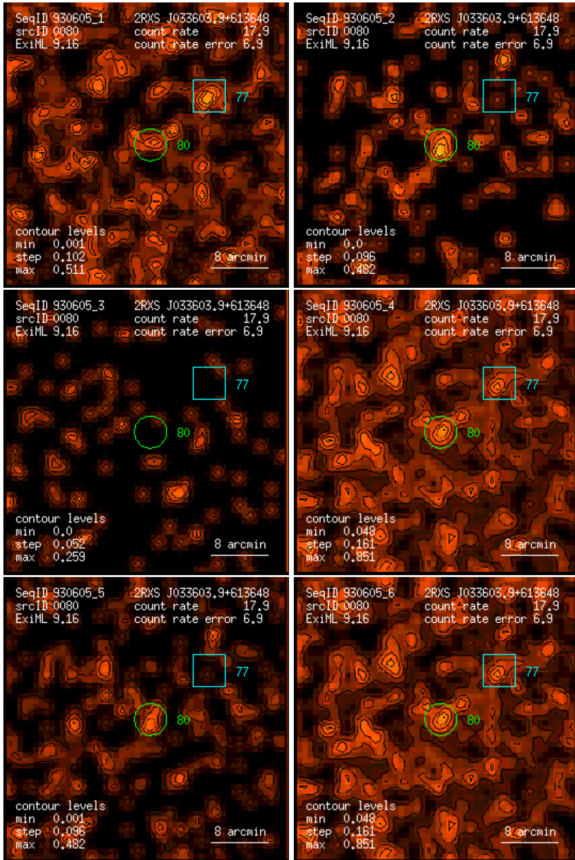
Figure 80: RASS 930605: detection 0080: band rate images, Gaussian filter: (1) PSPC channels 11 – 41, (2) 52 – 90, (3) 91 – 201, (4) 11 – 235, (5) 52 – 201, (6) 11 – 201. Broad band rates in counts/ks. Band rate contour levels in counts/ks/arcmin 2 .
