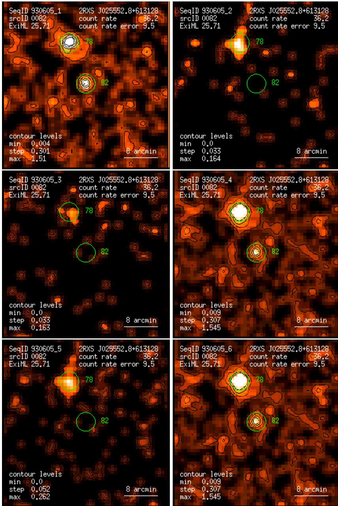
Figure 82: RASS 930605: detection 0082: band rate images, Gaussian filter: (1) PSPC channels 11 – 41, (2) 52 – 90, (3) 91 – 201, (4) 11 – 235, (5) 52 – 201, (6) 11 – 201. Broad band rates in counts/ks. Band rate contour levels in counts/ks/arcmin 2 .
