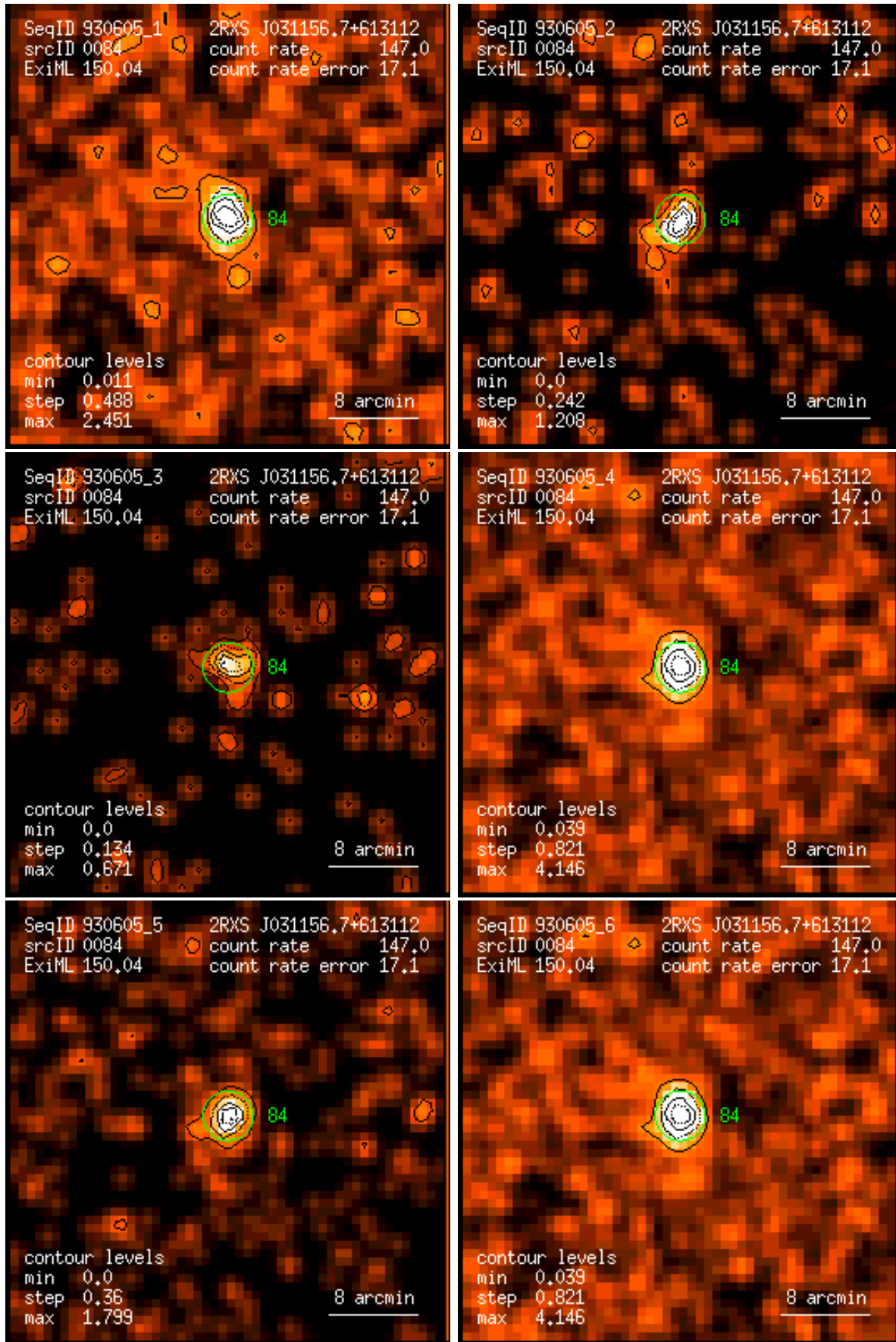
Figure 84: RASS 930605: detection 0084: band rate images, Gaussian filter: (1) PSPC channels 11 – 41, (2) 52 – 90, (3) 91 – 201, (4) 11 – 235, (5) 52 – 201, (6) 11 – 201. Broad band rates in counts/ks. Band rate contour levels in counts/ks/arcmin 2 .
