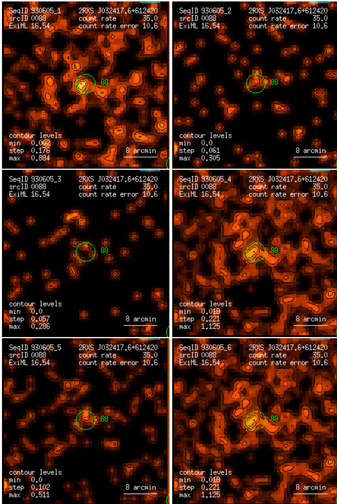
Figure 88: RASS 930605: detection 0088: band rate images, Gaussian filter: (1) PSPC channels 11 – 41, (2) 52 – 90, (3) 91 – 201, (4) 11 – 235, (5) 52 – 201, (6) 11 – 201. Broad band rates in counts/ks. Band rate contour levels in counts/ks/arcmin 2 .
