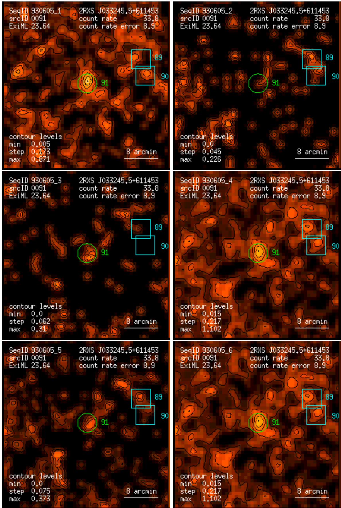
Figure 91: RASS 930605: detection 0091: band rate images, Gaussian filter: (1) PSPC channels 11 – 41, (2) 52 – 90, (3) 91 – 201, (4) 11 – 235, (5) 52 – 201, (6) 11 – 201. Broad band rates in counts/ks. Band rate contour levels in counts/ks/arcmin 2 .
