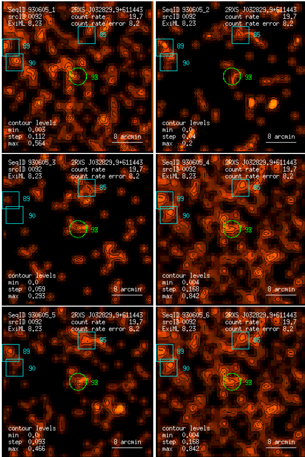
Figure 92: RASS 930605: detection 0092: band rate images, Gaussian filter: (1) PSPC channels 11 – 41, (2) 52 – 90, (3) 91 – 201, (4) 11 – 235, (5) 52 – 201, (6) 11 – 201. Broad band rates in counts/ks. Band rate contour levels in counts/ks/arcmin 2 .
