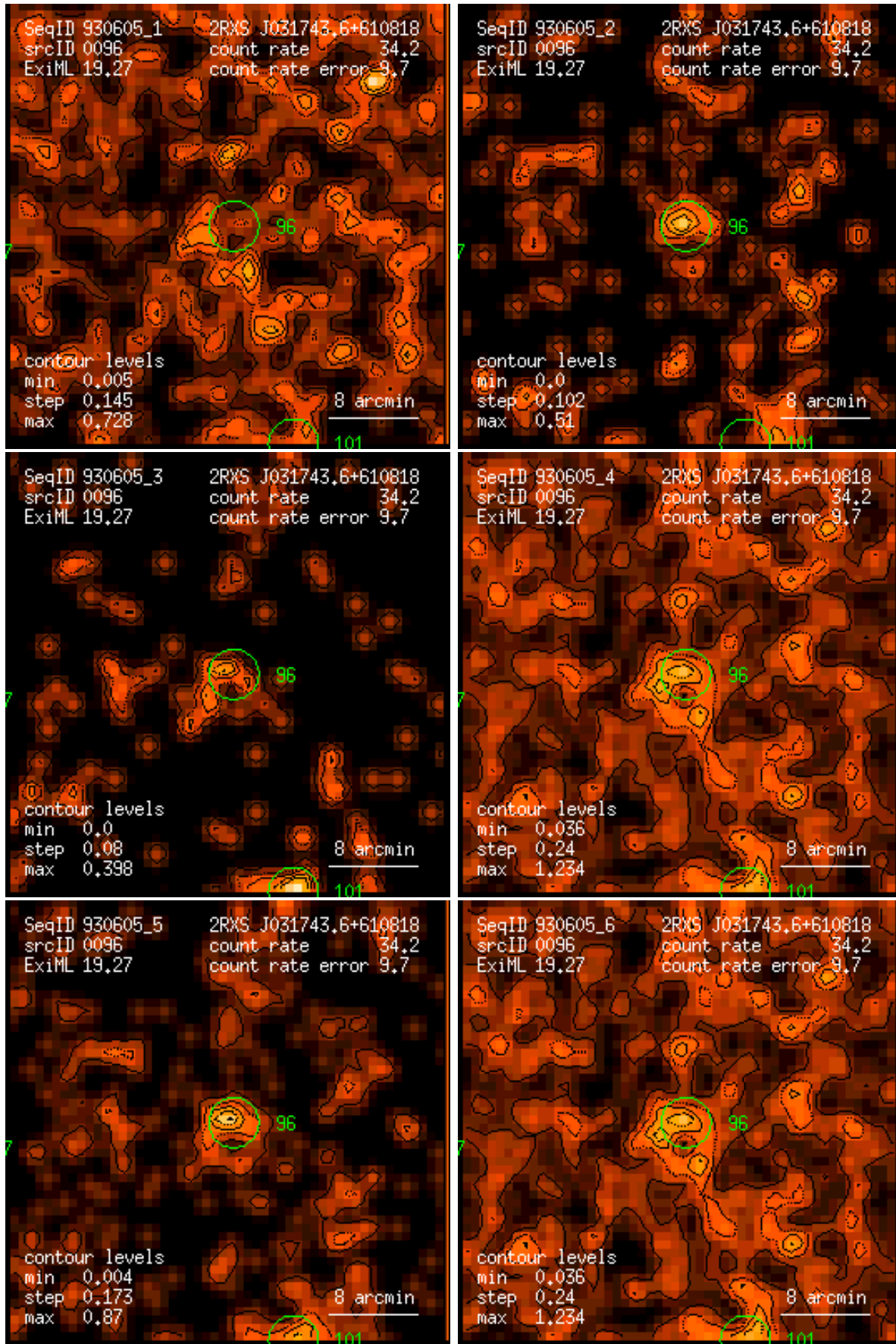
Figure 96: RASS 930605: detection 0096: band rate images, Gaussian filter: (1) PSPC channels 11 – 41, (2) 52 – 90, (3) 91 – 201, (4) 11 – 235, (5) 52 – 201, (6) 11 – 201. Broad band rates in counts/ks. Band rate contour levels in counts/ks/arcmin 2 .
