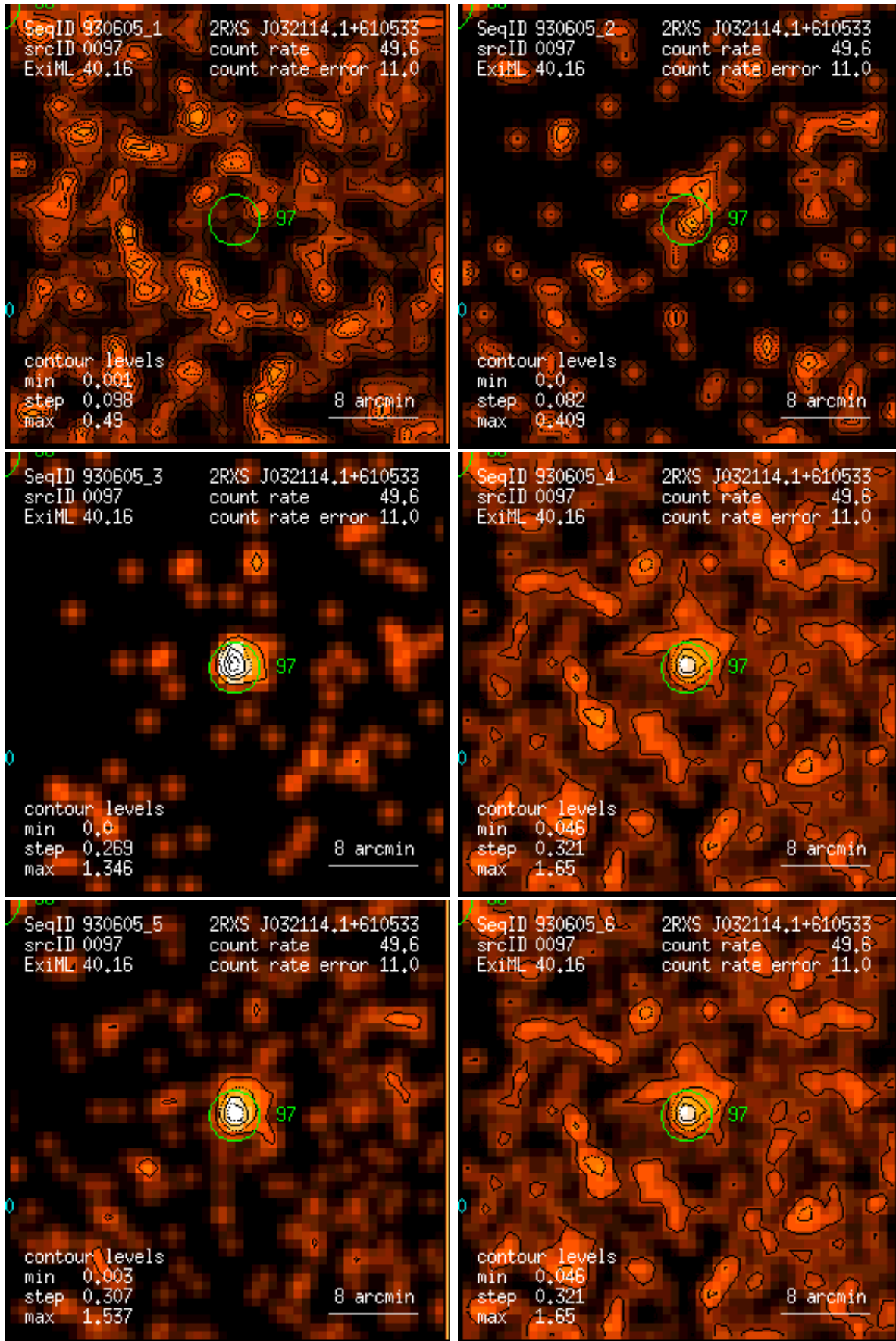
Figure 97: RASS 930605: detection 0097: band rate images, Gaussian filter: (1) PSPC channels 11 – 41, (2) 52 – 90, (3) 91 – 201, (4) 11 – 235, (5) 52 – 201, (6) 11 – 201. Broad band rates in counts/ks. Band rate contour levels in counts/ks/arcmin 2 .
