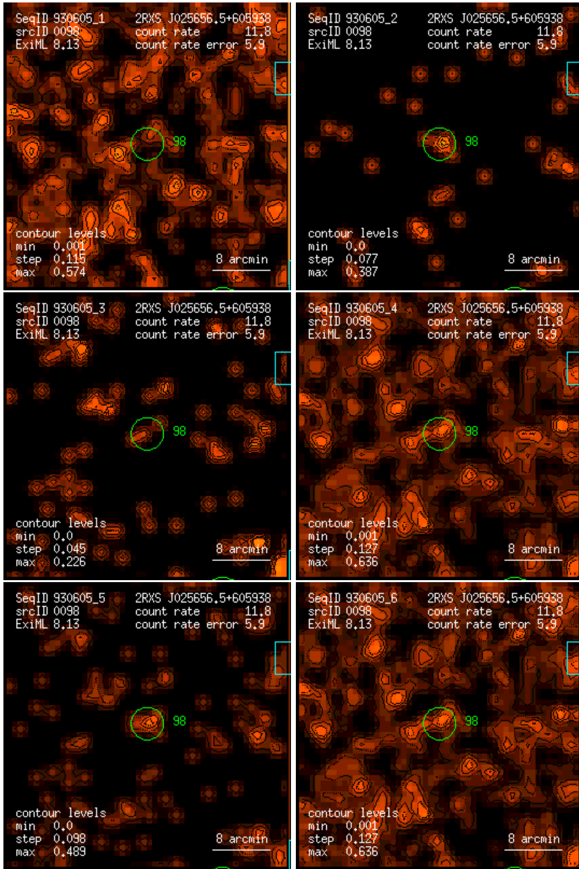
Figure 98: RASS 930605: detection 0098: band rate images, Gaussian filter: (1) PSPC channels 11 – 41, (2) 52 – 90, (3) 91 – 201, (4) 11 – 235, (5) 52 – 201, (6) 11 – 201. Broad band rates in counts/ks. Band rate contour levels in counts/ks/arcmin 2 .
