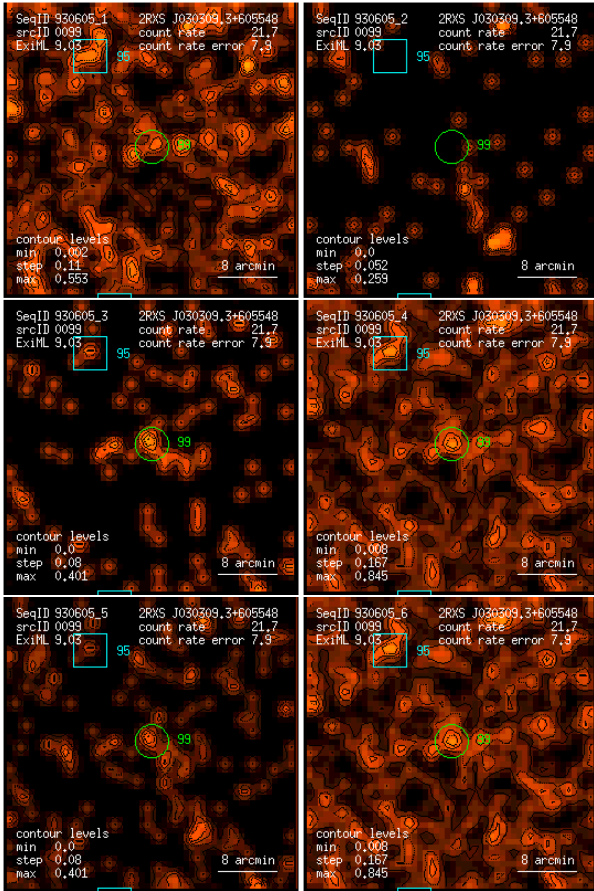
Figure 99: RASS 930605: detection 0099: band rate images, Gaussian filter: (1) PSPC channels 11 – 41, (2) 52 – 90, (3) 91 – 201, (4) 11 – 235, (5) 52 – 201, (6) 11 – 201. Broad band rates in counts/ks. Band rate contour levels in counts/ks/arcmin 2 .
