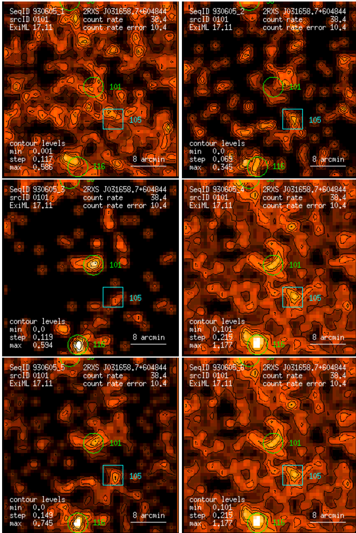
Figure 101: RASS 930605: detection 0101: band rate images, Gaussian filter: (1) PSPC channels 11 – 41, (2) 52 – 90, (3) 91 – 201, (4) 11 – 235, (5) 52 – 201, (6) 11 – 201. Broad band rates in counts/ks. Band rate contour levels in counts/ks/arcmin 2 .
