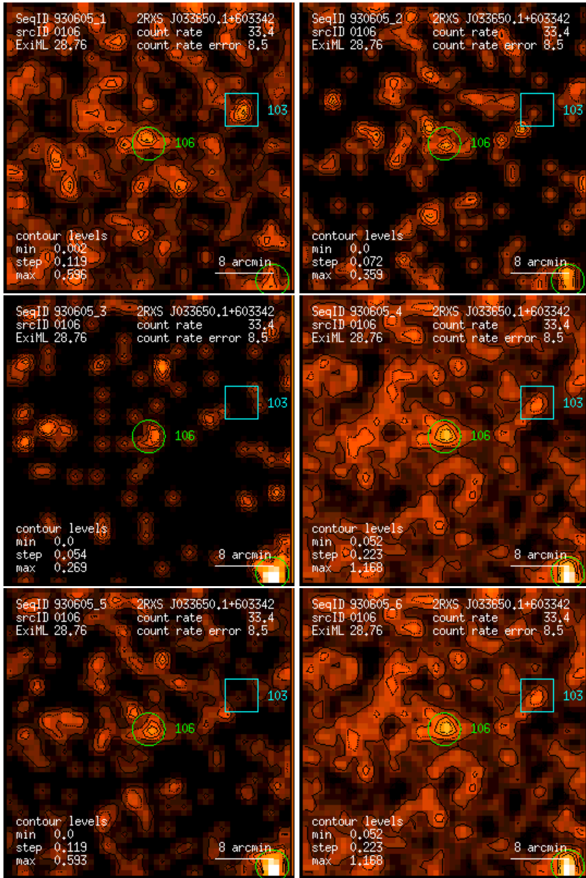
Figure 106: RASS 930605: detection 0106: band rate images, Gaussian filter: (1) PSPC channels 11 – 41, (2) 52 – 90, (3) 91 – 201, (4) 11 – 235, (5) 52 – 201, (6) 11 – 201. Broad band rates in counts/ks. Band rate contour levels in counts/ks/arcmin 2 .
