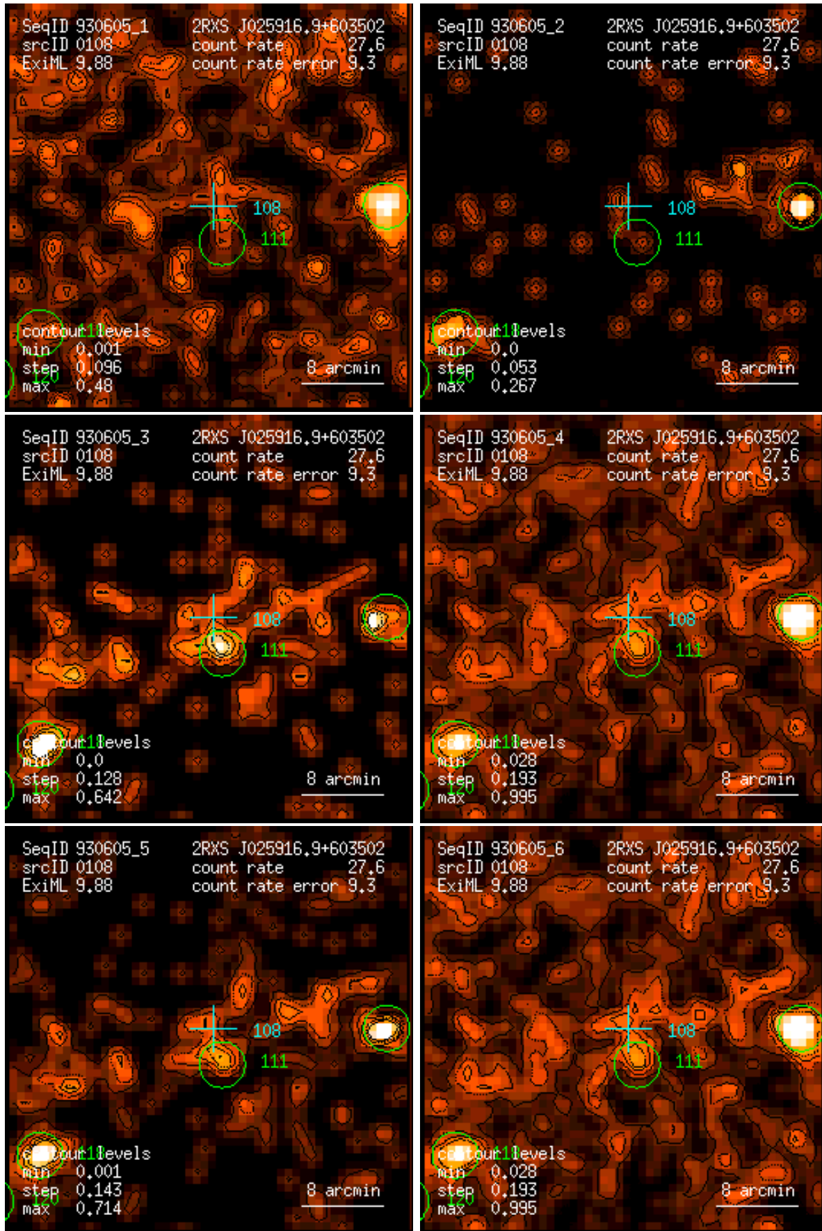
Figure 108: RASS 930605: detection 0108: band rate images, Gaussian filter: (1) PSPC channels 11 – 41, (2) 52 – 90, (3) 91 – 201, (4) 11 – 235, (5) 52 – 201, (6) 11 – 201. Broad band rates in counts/ks. Band rate contour levels in counts/ks/arcmin 2 .
