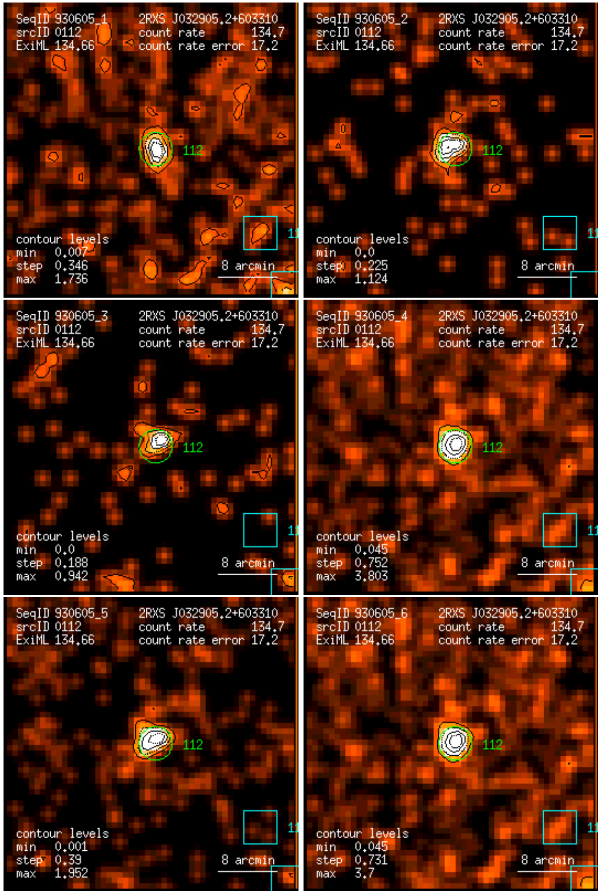
Figure 112: RASS 930605: detection 0112: band rate images, Gaussian filter: (1) PSPC channels 11 – 41, (2) 52 – 90, (3) 91 – 201, (4) 11 – 235, (5) 52 – 201, (6) 11 – 201. Broad band rates in counts/ks. Band rate contour levels in counts/ks/arcmin 2 .
