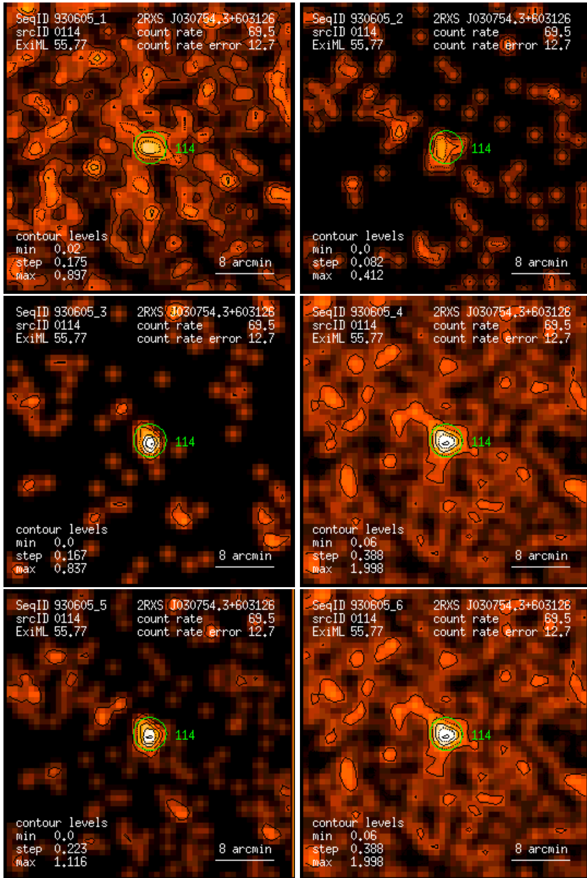
Figure 114: RASS 930605: detection 0114: band rate images, Gaussian filter: (1) PSPC channels 11 – 41, (2) 52 – 90, (3) 91 – 201, (4) 11 – 235, (5) 52 – 201, (6) 11 – 201. Broad band rates in counts/ks. Band rate contour levels in counts/ks/arcmin 2 .
