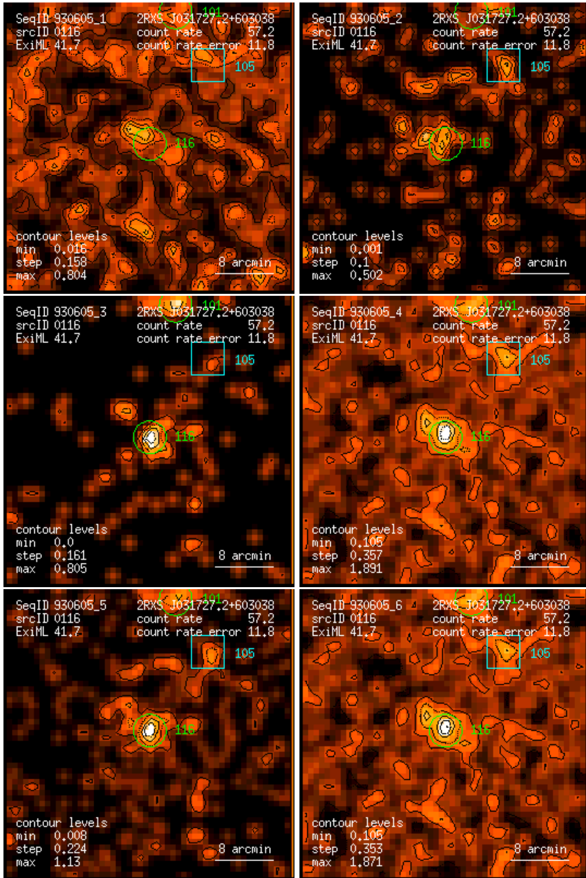
Figure 116: RASS 930605: detection 0116: band rate images, Gaussian filter: (1) PSPC channels 11 – 41, (2) 52 – 90, (3) 91 – 201, (4) 11 – 235, (5) 52 – 201, (6) 11 – 201. Broad band rates in counts/ks. Band rate contour levels in counts/ks/arcmin 2 .
