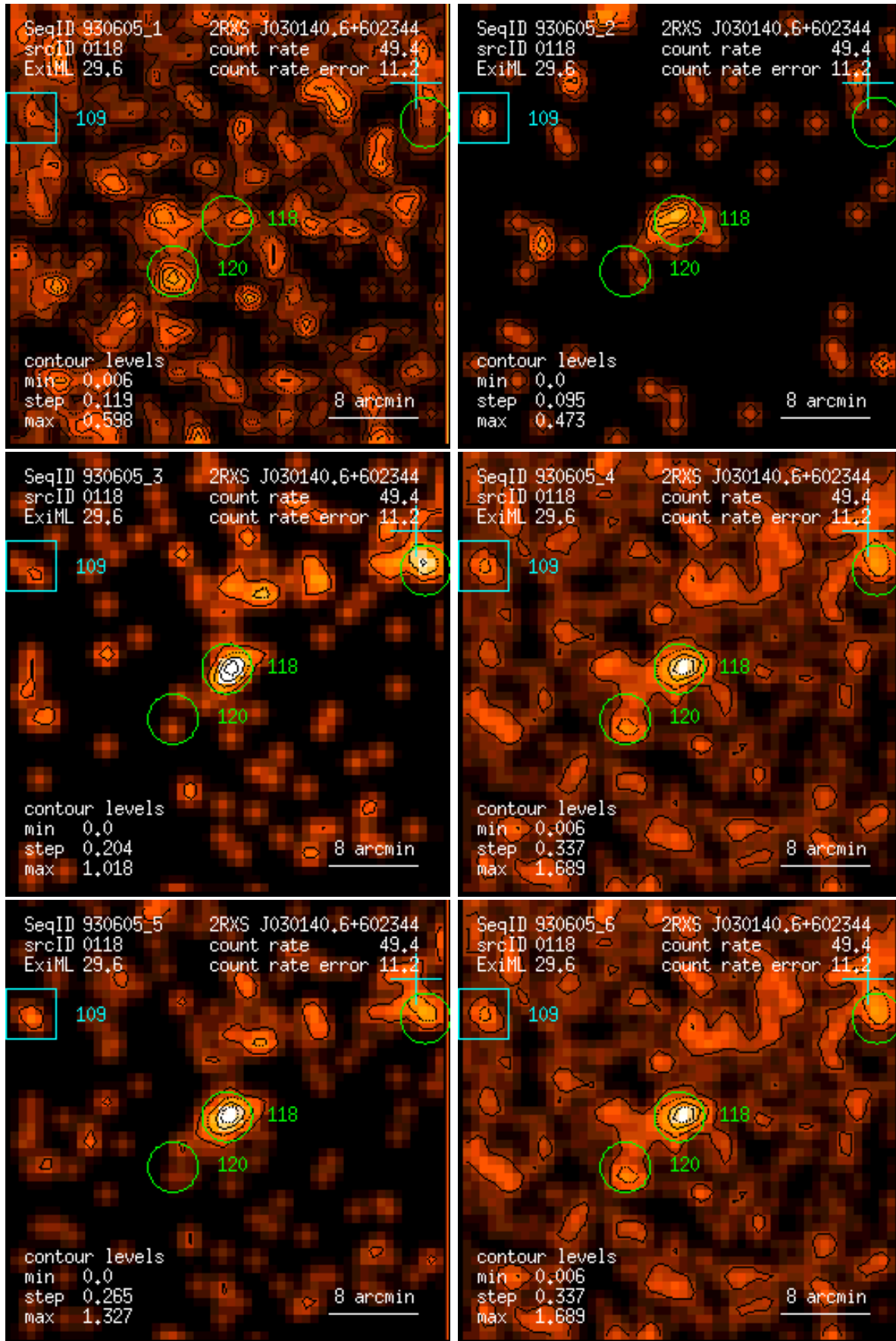
Figure 118: RASS 930605: detection 0118: band rate images, Gaussian filter: (1) PSPC channels 11 – 41, (2) 52 – 90, (3) 91 – 201, (4) 11 – 235, (5) 52 – 201, (6) 11 – 201. Broad band rates in counts/ks. Band rate contour levels in counts/ks/arcmin 2 .
