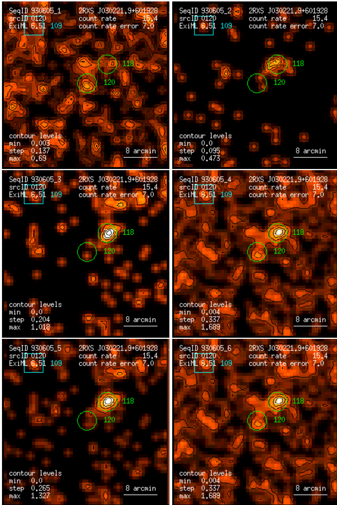
Figure 120: RASS 930605: detection 0120: band rate images, Gaussian filter: (1) PSPC channels 11 – 41, (2) 52 – 90, (3) 91 – 201, (4) 11 – 235, (5) 52 – 201, (6) 11 – 201. Broad band rates in counts/ks. Band rate contour levels in counts/ks/arcmin 2 .
