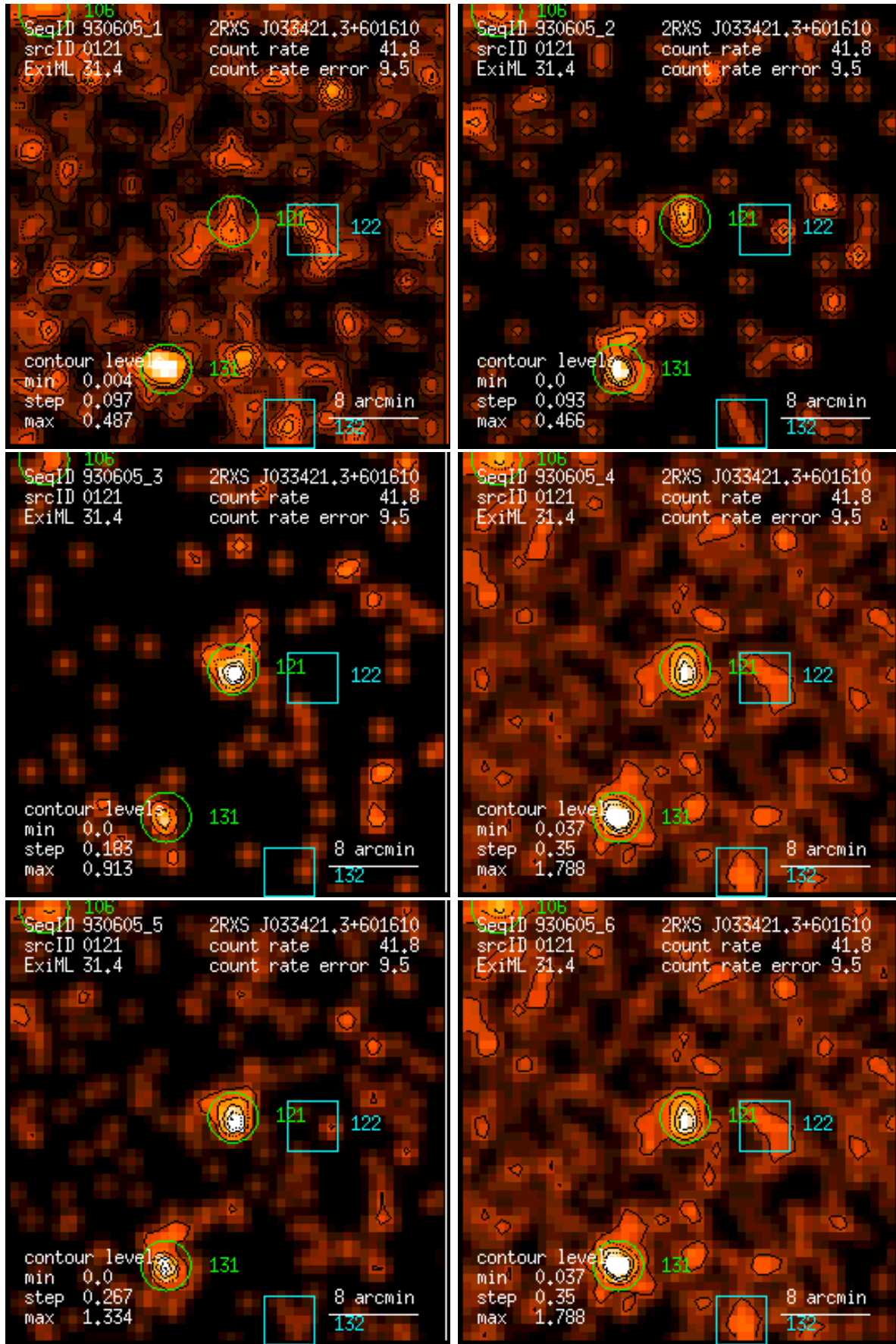
Figure 121: RASS 930605: detection 0121: band rate images, Gaussian filter: (1) PSPC channels 11 – 41, (2) 52 – 90, (3) 91 – 201, (4) 11 – 235, (5) 52 – 201, (6) 11 – 201. Broad band rates in counts/ks. Band rate contour levels in counts/ks/arcmin 2 .
