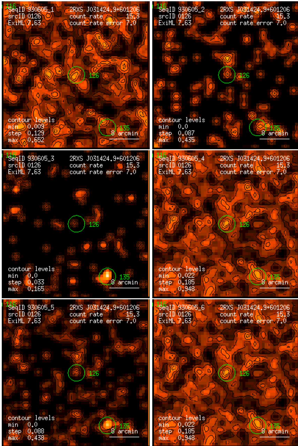
Figure 126: RASS 930605: detection 0126: band rate images, Gaussian filter: (1) PSPC channels 11 – 41, (2) 52 – 90, (3) 91 – 201, (4) 11 – 235, (5) 52 – 201, (6) 11 – 201. Broad band rates in counts/ks. Band rate contour levels in counts/ks/arcmin 2 .
