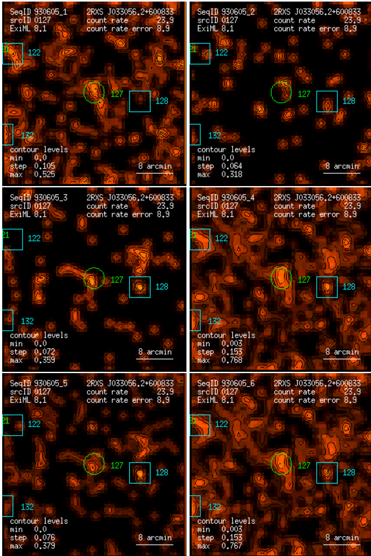
Figure 127: RASS 930605: detection 0127: band rate images, Gaussian filter: (1) PSPC channels 11 – 41, (2) 52 – 90, (3) 91 – 201, (4) 11 – 235, (5) 52 – 201, (6) 11 – 201. Broad band rates in counts/ks. Band rate contour levels in counts/ks/arcmin 2 .
