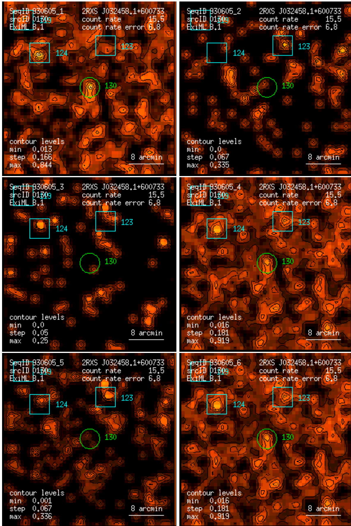
Figure 130: RASS 930605: detection 0130: band rate images, Gaussian filter: (1) PSPC channels 11 – 41, (2) 52 – 90, (3) 91 – 201, (4) 11 – 235, (5) 52 – 201, (6) 11 – 201. Broad band rates in counts/ks. Band rate contour levels in counts/ks/arcmin 2 .
