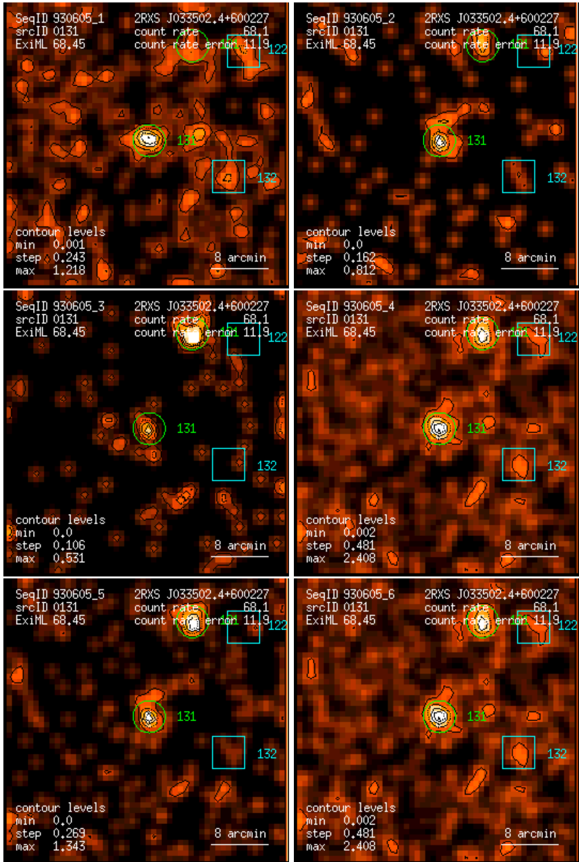
Figure 131: RASS 930605: detection 0131: band rate images, Gaussian filter: (1) PSPC channels 11 – 41, (2) 52 – 90, (3) 91 – 201, (4) 11 – 235, (5) 52 – 201, (6) 11 – 201. Broad band rates in counts/ks. Band rate contour levels in counts/ks/arcmin 2 .
