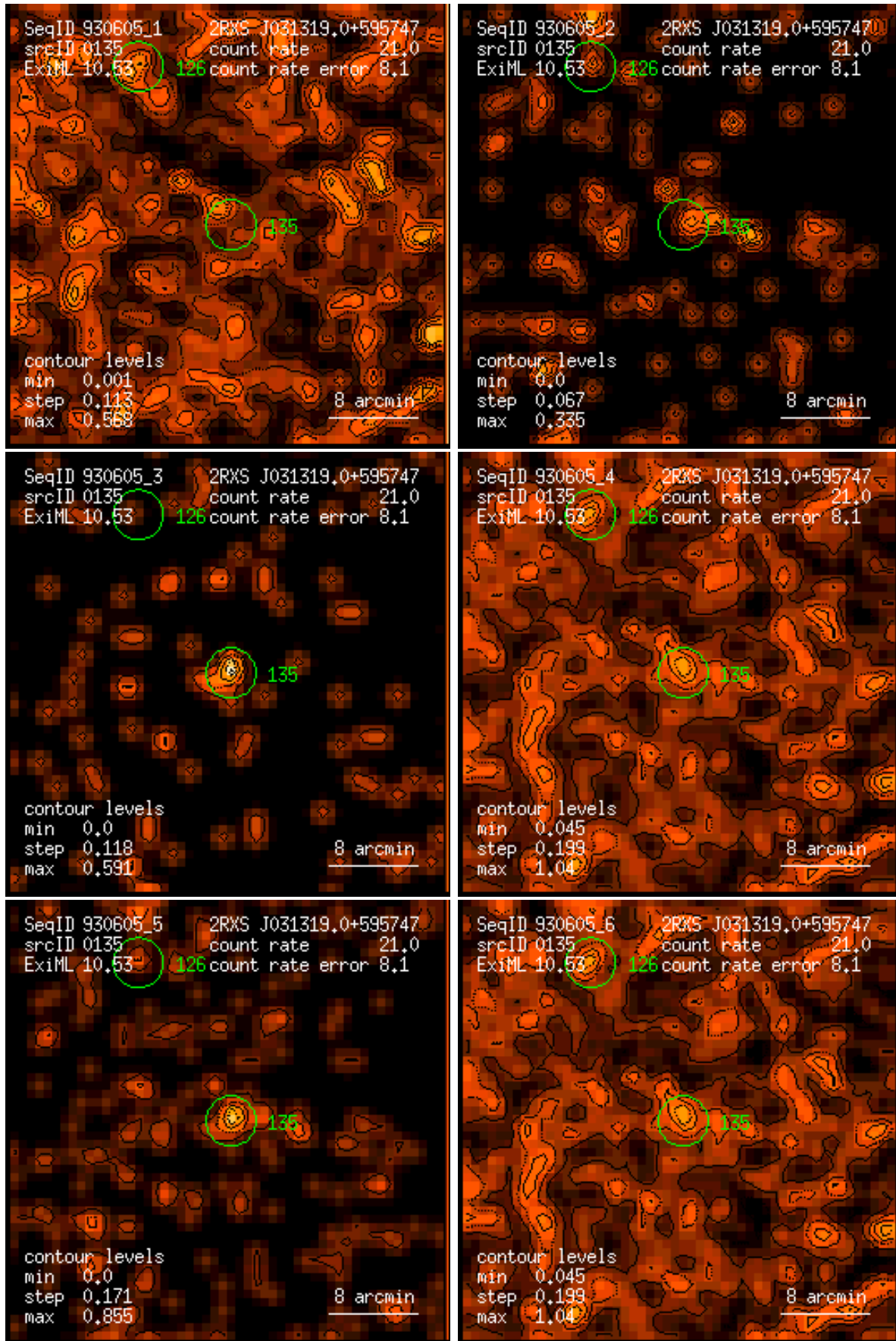
Figure 135: RASS 930605: detection 0135: band rate images, Gaussian filter: (1) PSPC channels 11 – 41, (2) 52 – 90, (3) 91 – 201, (4) 11 – 235, (5) 52 – 201, (6) 11 – 201. Broad band rates in counts/ks. Band rate contour levels in counts/ks/arcmin 2 .
