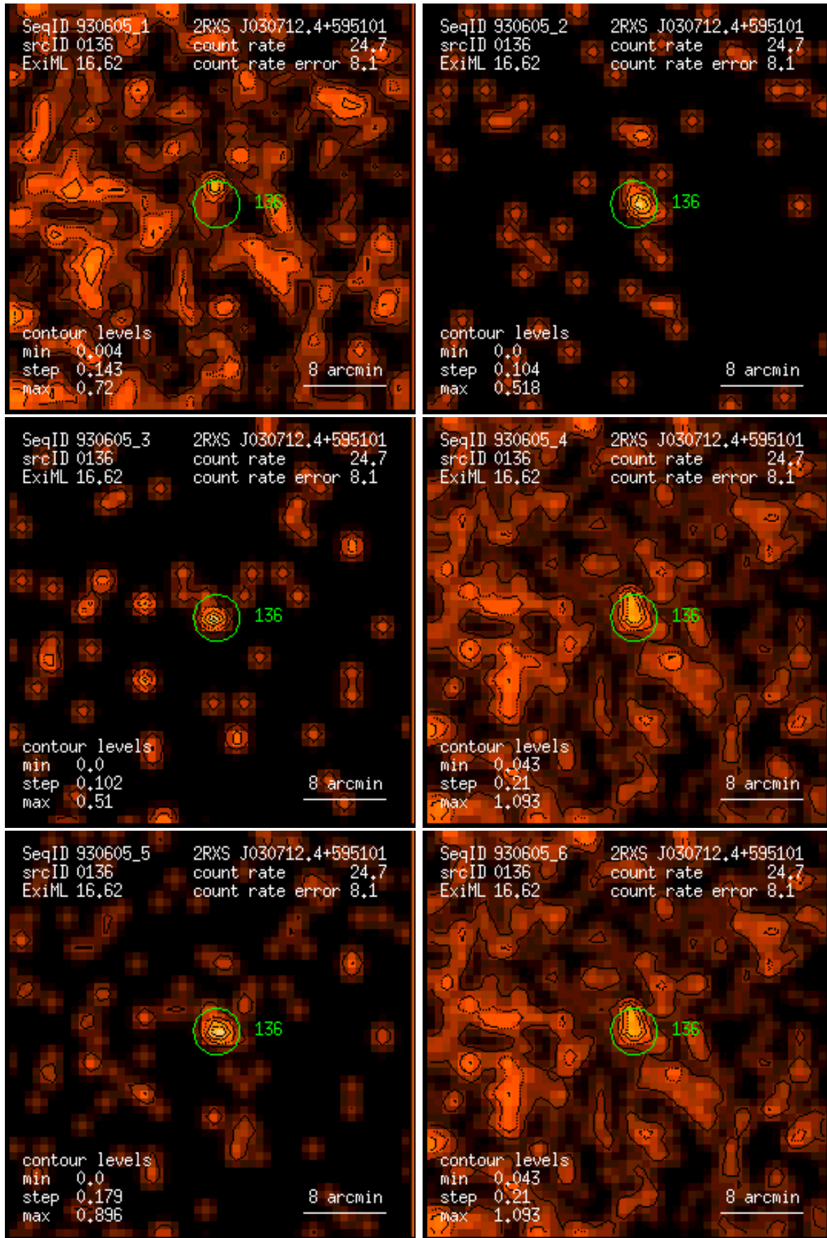
Figure 136: RASS 930605: detection 0136: band rate images, Gaussian filter: (1) PSPC channels 11 – 41, (2) 52 – 90, (3) 91 – 201, (4) 11 – 235, (5) 52 – 201, (6) 11 – 201. Broad band rates in counts/ks. Band rate contour levels in counts/ks/arcmin 2 .
