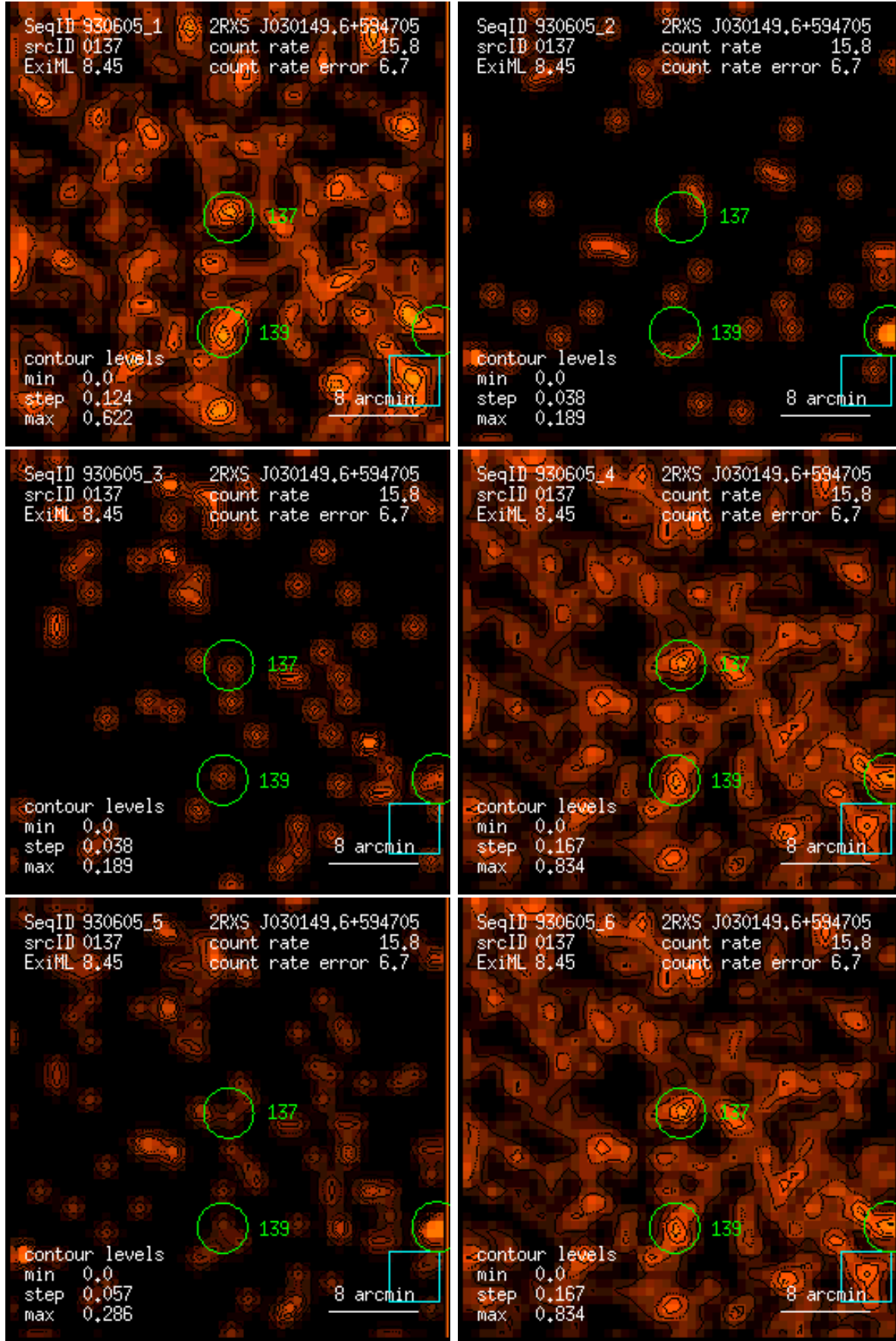
Figure 137: RASS 930605: detection 0137: band rate images, Gaussian filter: (1) PSPC channels 11 – 41, (2) 52 – 90, (3) 91 – 201, (4) 11 – 235, (5) 52 – 201, (6) 11 – 201. Broad band rates in counts/ks. Band rate contour levels in counts/ks/arcmin 2 .
