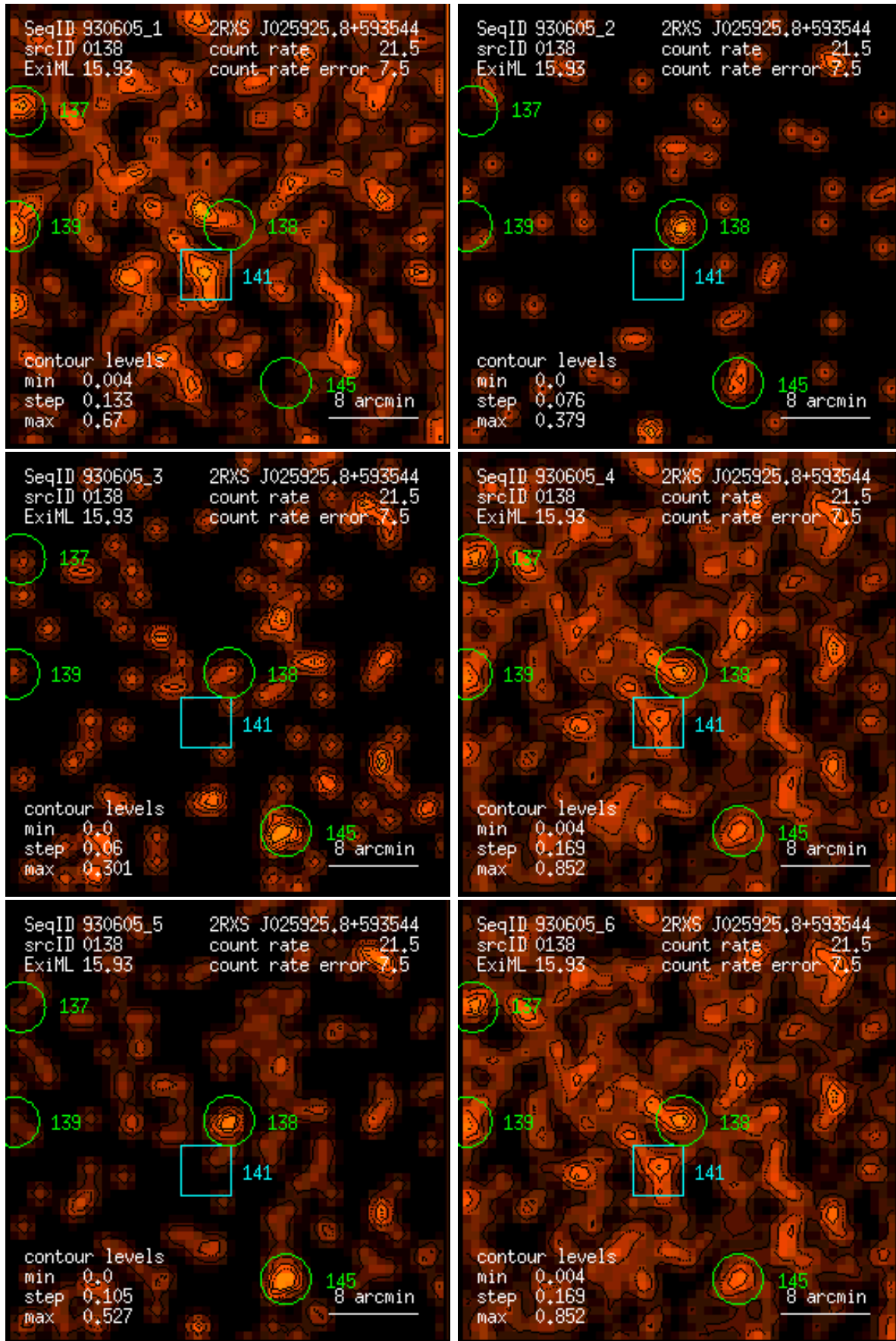
Figure 138: RASS 930605: detection 0138: band rate images, Gaussian filter: (1) PSPC channels 11 – 41, (2) 52 – 90, (3) 91 – 201, (4) 11 – 235, (5) 52 – 201, (6) 11 – 201. Broad band rates in counts/ks. Band rate contour levels in counts/ks/arcmin 2 .
