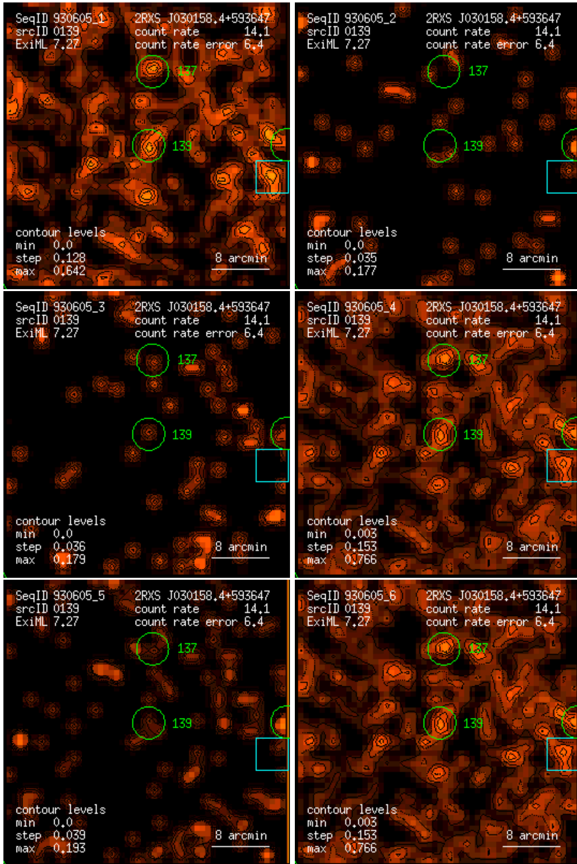
Figure 139: RASS 930605: detection 0139: band rate images, Gaussian filter: (1) PSPC channels 11 – 41, (2) 52 – 90, (3) 91 – 201, (4) 11 – 235, (5) 52 – 201, (6) 11 – 201. Broad band rates in counts/ks. Band rate contour levels in counts/ks/arcmin 2 .
