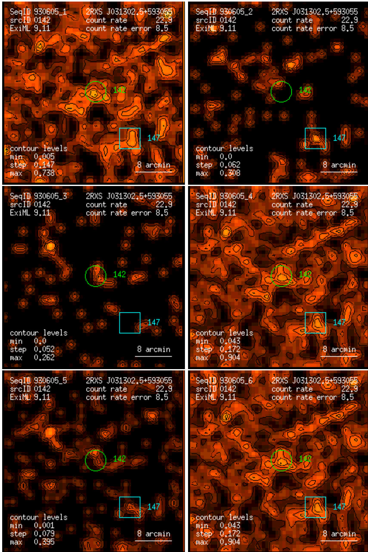
Figure 142: RASS 930605: detection 0142: band rate images, Gaussian filter: (1) PSPC channels 11 – 41, (2) 52 – 90, (3) 91 – 201, (4) 11 – 235, (5) 52 – 201, (6) 11 – 201. Broad band rates in counts/ks. Band rate contour levels in counts/ks/arcmin 2 .
