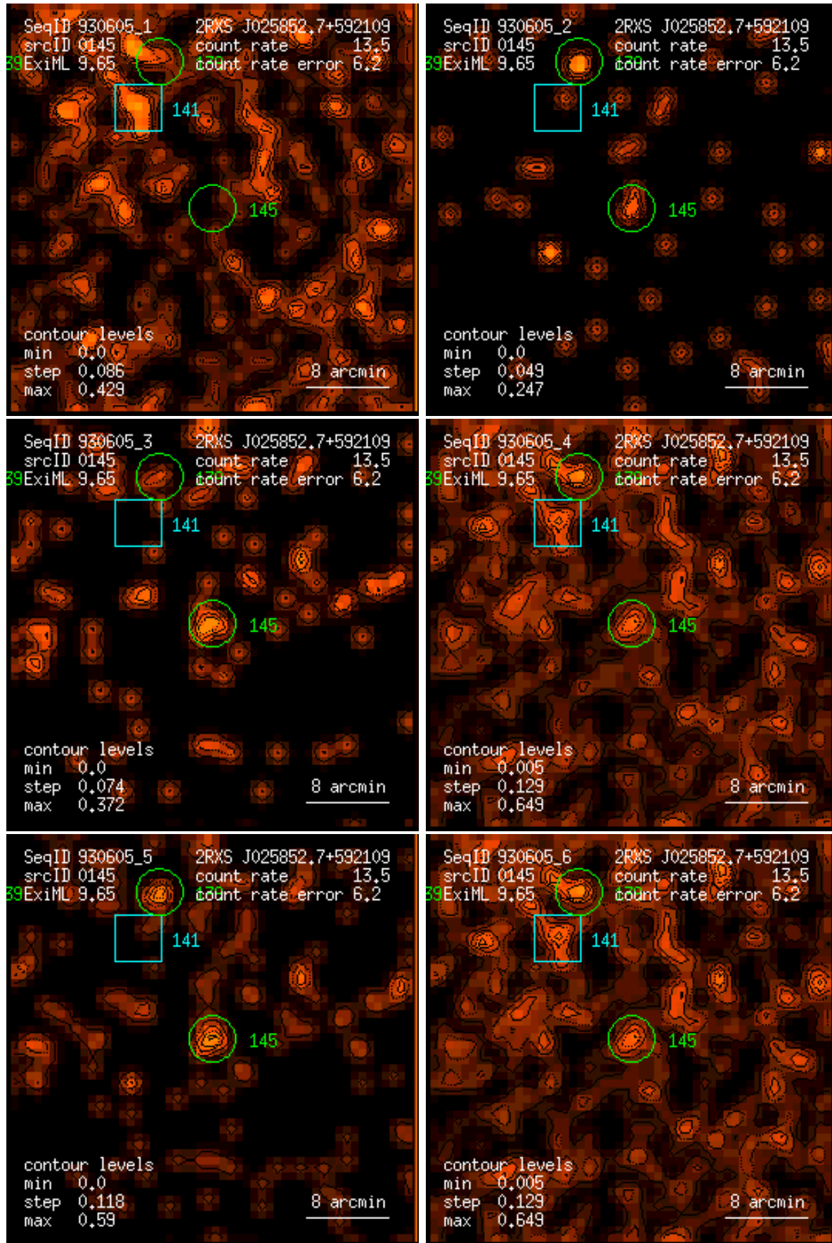
Figure 145: RASS 930605: detection 0145: band rate images, Gaussian filter: (1) PSPC channels 11 – 41, (2) 52 – 90, (3) 91 – 201, (4) 11 – 235, (5) 52 – 201, (6) 11 – 201. Broad band rates in counts/ks. Band rate contour levels in counts/ks/arcmin 2 .
