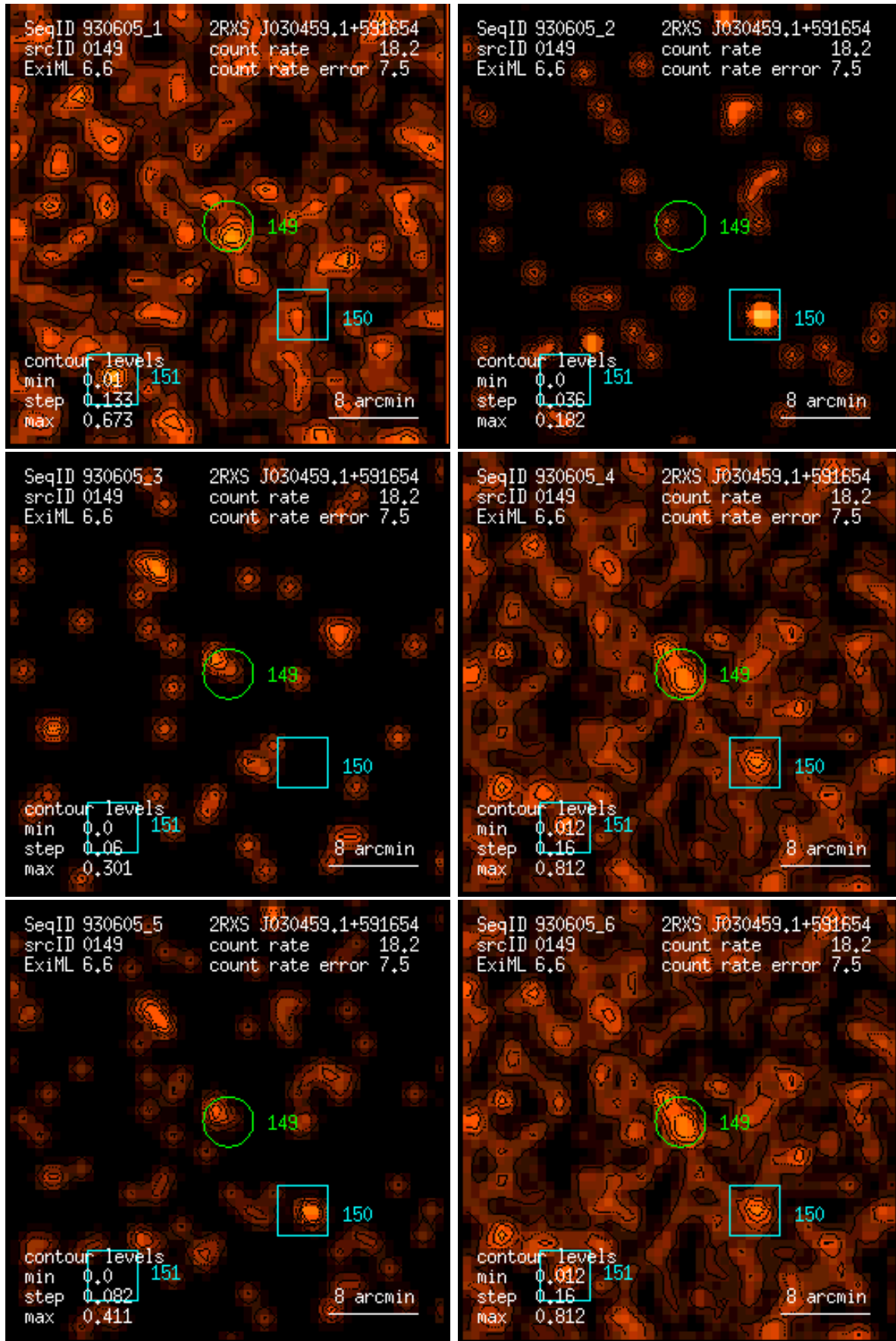
Figure 149: RASS 930605: detection 0149: band rate images, Gaussian filter: (1) PSPC channels 11 – 41, (2) 52 – 90, (3) 91 – 201, (4) 11 – 235, (5) 52 – 201, (6) 11 – 201. Broad band rates in counts/ks. Band rate contour levels in counts/ks/arcmin 2 .
