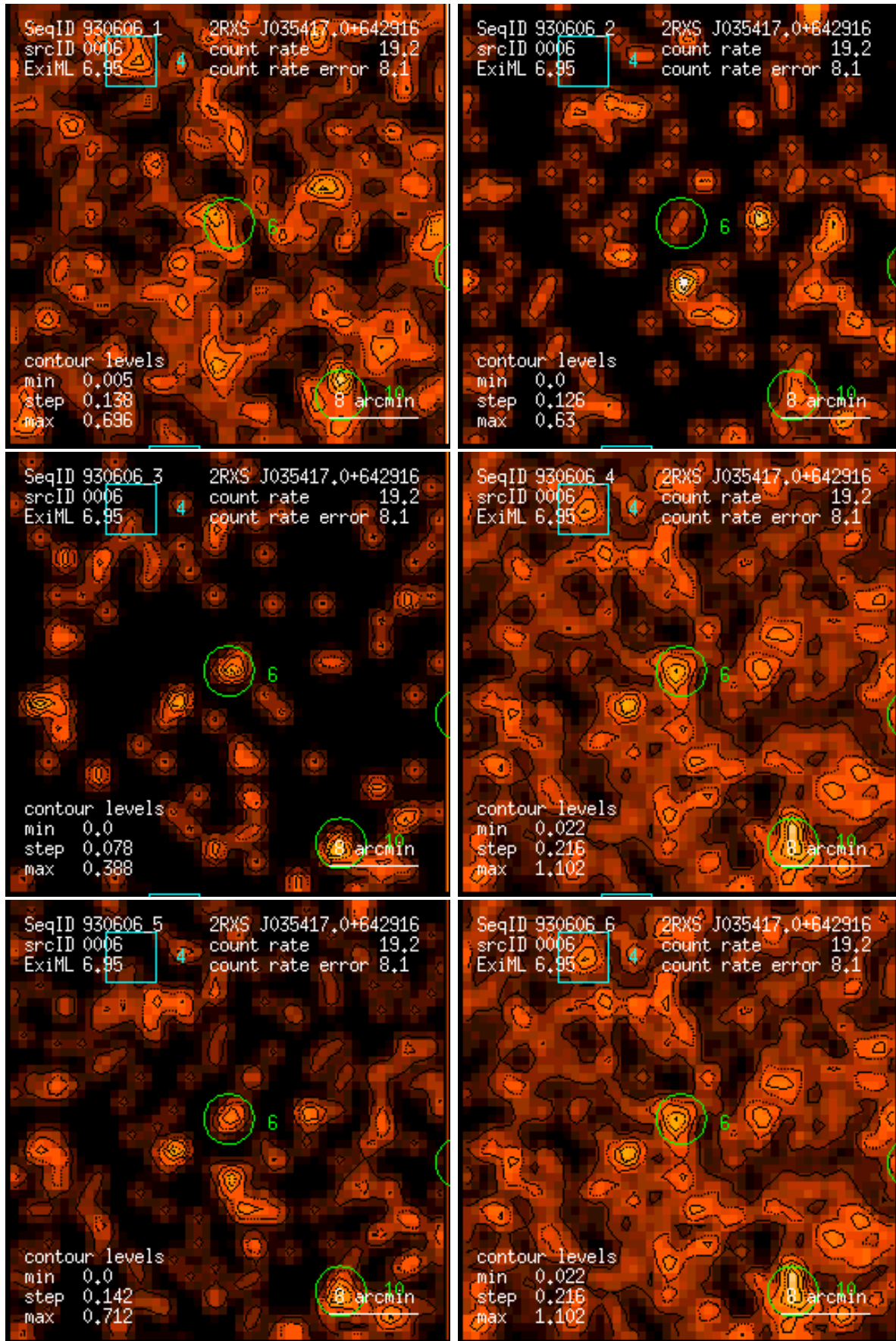
Figure 6: RASS 930606: detection 0006: band rate images, Gaussian filter: (1) PSPC channels 11 – 41, (2) 52 – 90, (3) 91 – 201, (4) 11 – 235, (5) 52 – 201, (6) 11 – 201. Broad band rates in counts/ks. Band rate contour levels in counts/ks/arcmin 2 .
