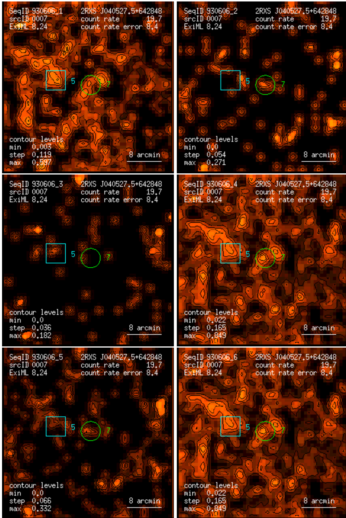
Figure 7: RASS 930606: detection 0007: band rate images, Gaussian filter: (1) PSPC channels 11 – 41, (2) 52 – 90, (3) 91 – 201, (4) 11 – 235, (5) 52 – 201, (6) 11 – 201. Broad band rates in counts/ks. Band rate contour levels in counts/ks/arcmin 2 .
