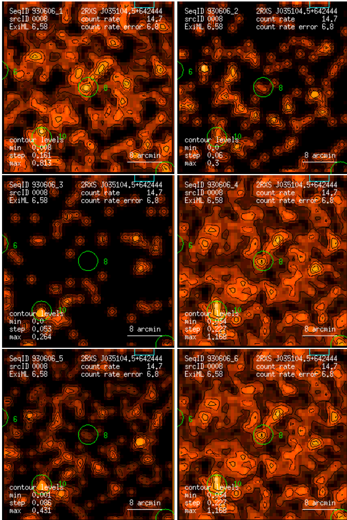
Figure 8: RASS 930606: detection 0008: band rate images, Gaussian filter: (1) PSPC channels 11 – 41, (2) 52 – 90, (3) 91 – 201, (4) 11 – 235, (5) 52 – 201, (6) 11 – 201. Broad band rates in counts/ks. Band rate contour levels in counts/ks/arcmin 2 .
