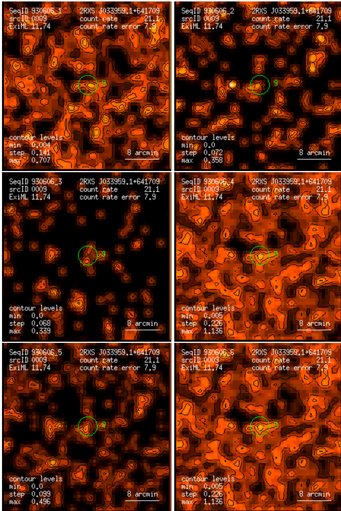
Figure 9: RASS 930606: detection 0009: band rate images, Gaussian filter: (1) PSPC channels 11 – 41, (2) 52 – 90, (3) 91 – 201, (4) 11 – 235, (5) 52 – 201, (6) 11 – 201. Broad band rates in counts/ks. Band rate contour levels in counts/ks/arcmin 2 .
