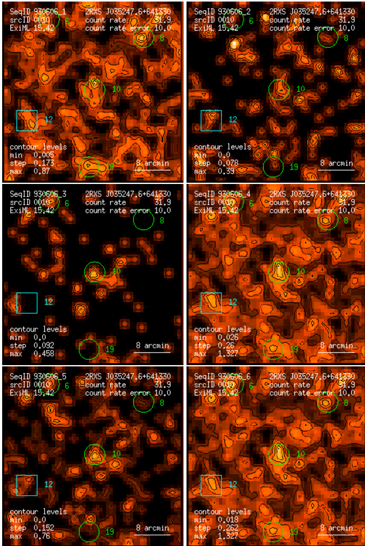
Figure 10: RASS 930606: detection 0010: band rate images, Gaussian filter: (1) PSPC channels 11 – 41, (2) 52 – 90, (3) 91 – 201, (4) 11 – 235, (5) 52 – 201, (6) 11 – 201. Broad band rates in counts/ks. Band rate contour levels in counts/ks/arcmin 2 .
