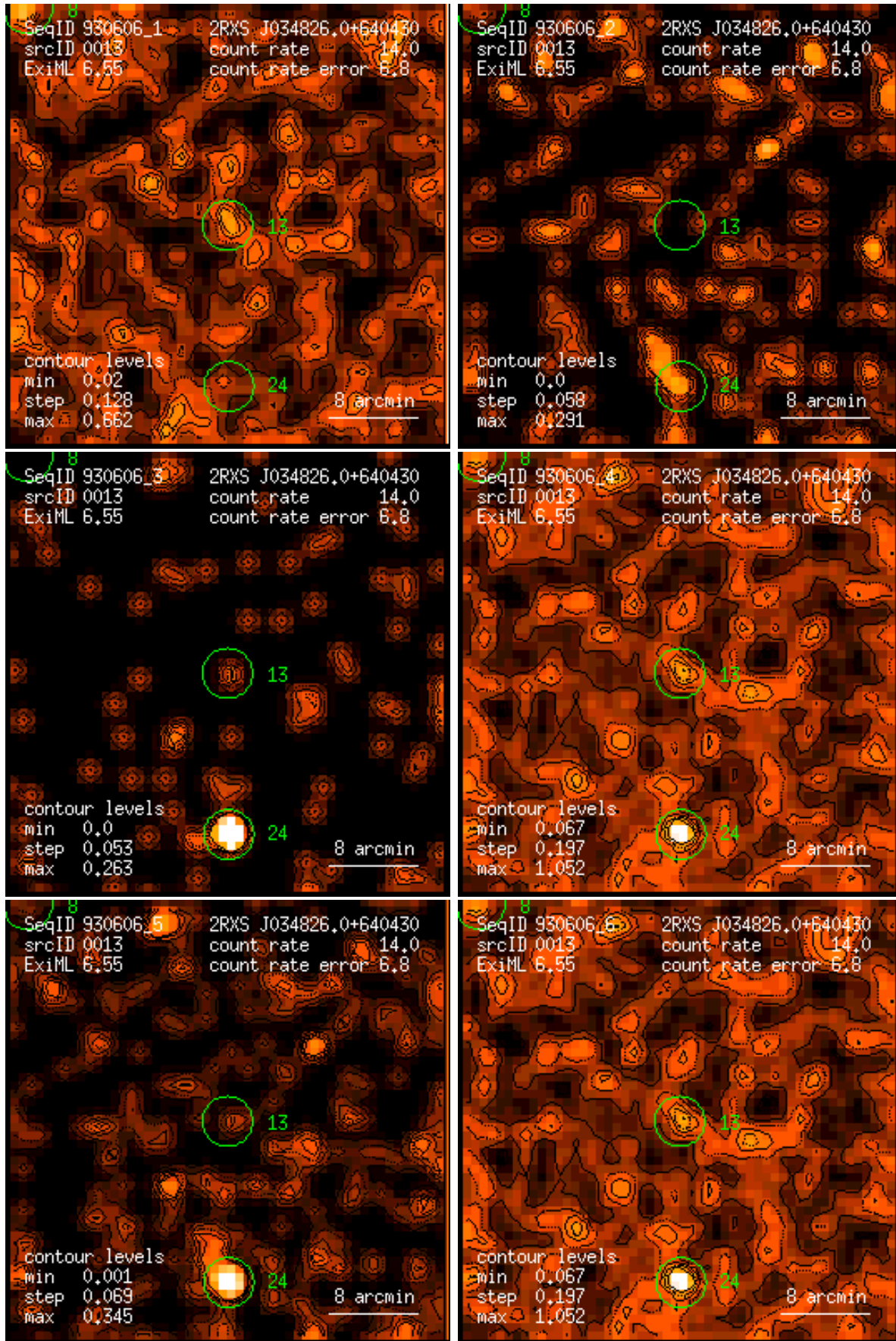
Figure 13: RASS 930606: detection 0013: band rate images, Gaussian filter: (1) PSPC channels 11 – 41, (2) 52 – 90, (3) 91 – 201, (4) 11 – 235, (5) 52 – 201, (6) 11 – 201. Broad band rates in counts/ks. Band rate contour levels in counts/ks/arcmin 2 .
