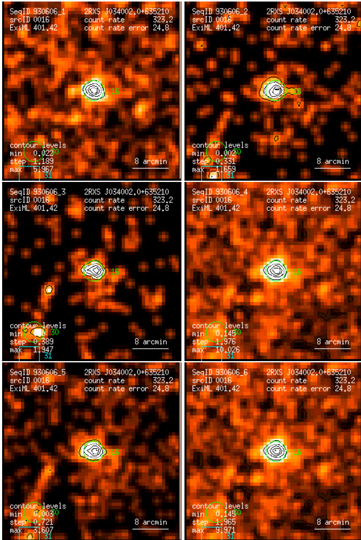
Figure 16: RASS 930606: detection 0016: band rate images, Gaussian filter: (1) PSPC channels 11 – 41, (2) 52 – 90, (3) 91 – 201, (4) 11 – 235, (5) 52 – 201, (6) 11 – 201. Broad band rates in counts/ks. Band rate contour levels in counts/ks/arcmin 2 .
