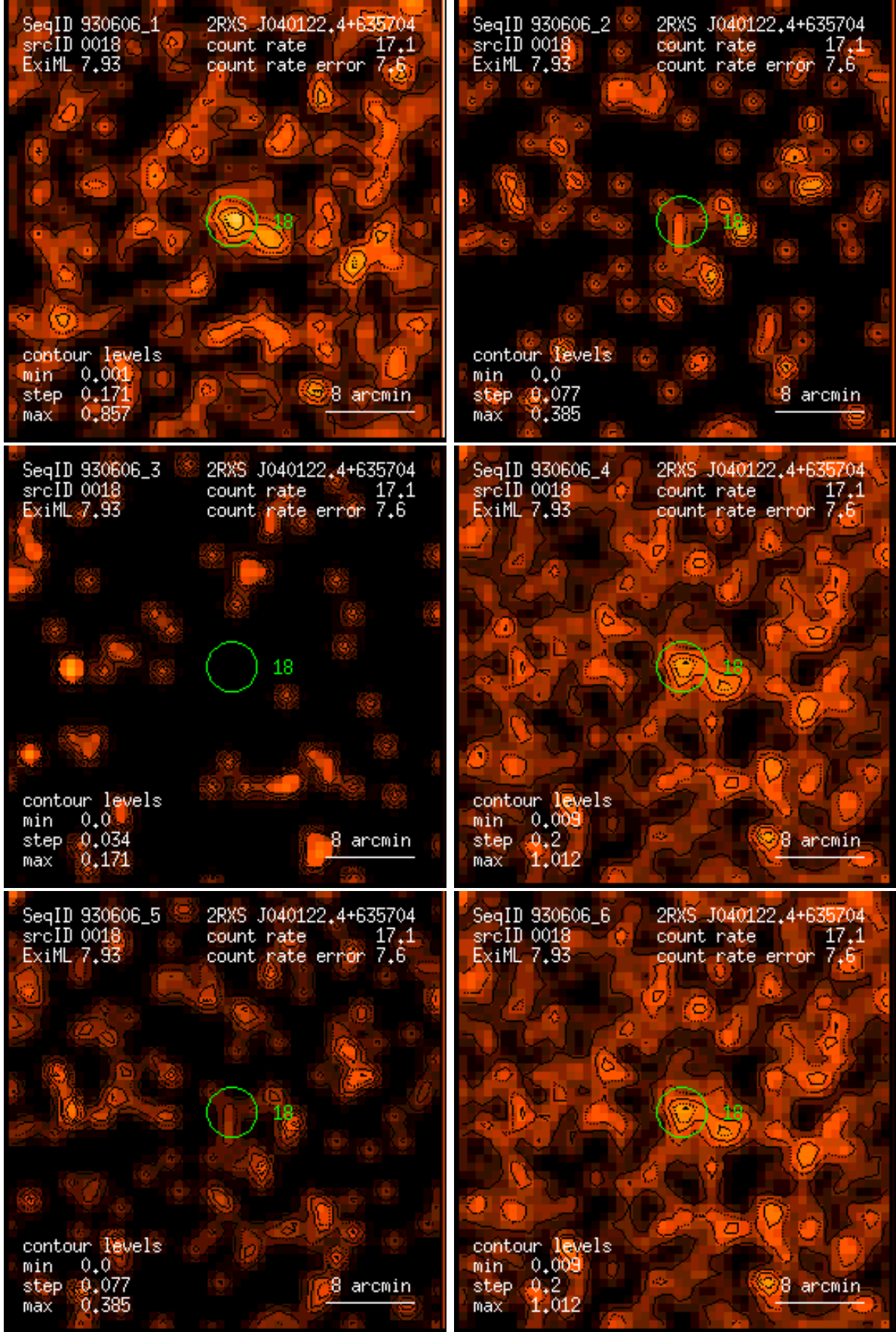
Figure 18: RASS 930606: detection 0018: band rate images, Gaussian filter: (1) PSPC channels 11 – 41, (2) 52 – 90, (3) 91 – 201, (4) 11 – 235, (5) 52 – 201, (6) 11 – 201. Broad band rates in counts/ks. Band rate contour levels in counts/ks/arcmin 2 .
