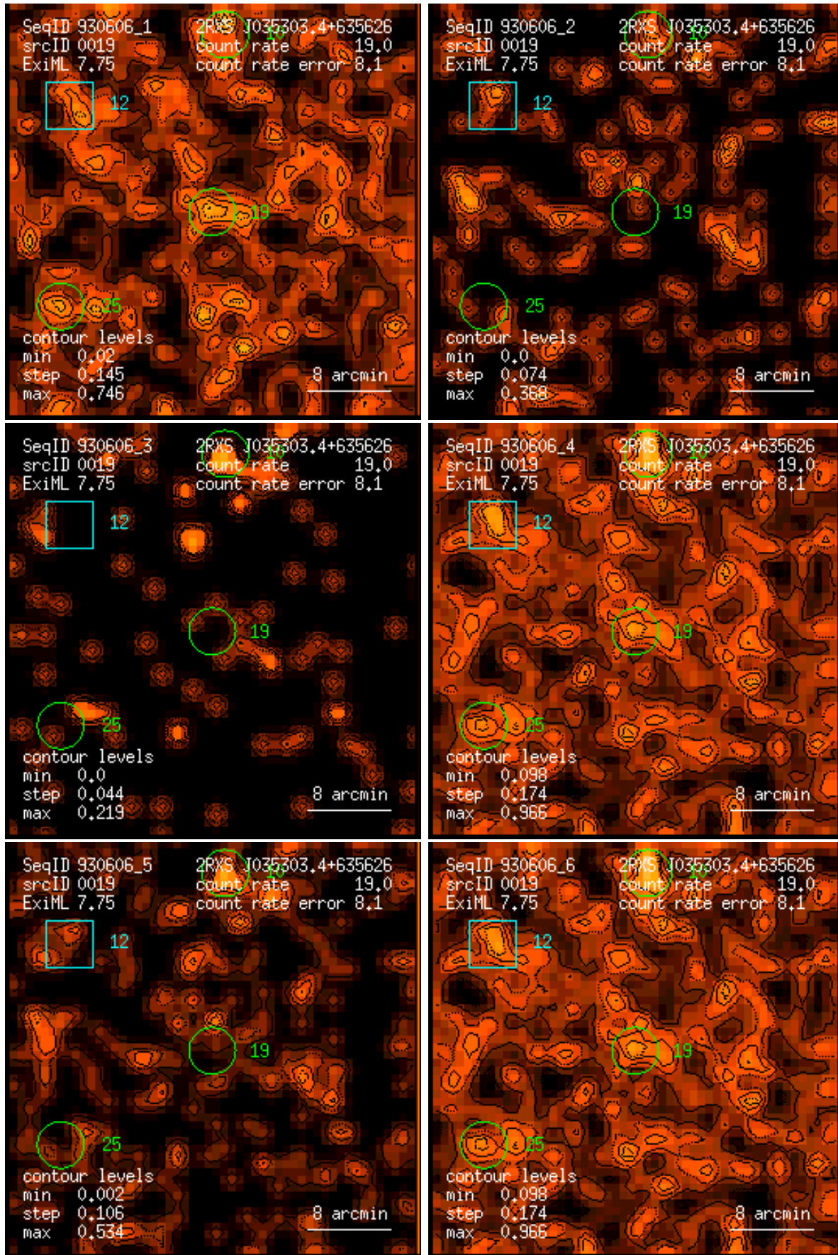
Figure 19: RASS 930606: detection 0019: band rate images, Gaussian filter: (1) PSPC channels 11 – 41, (2) 52 – 90, (3) 91 – 201, (4) 11 – 235, (5) 52 – 201, (6) 11 – 201. Broad band rates in counts/ks. Band rate contour levels in counts/ks/arcmin 2 .
