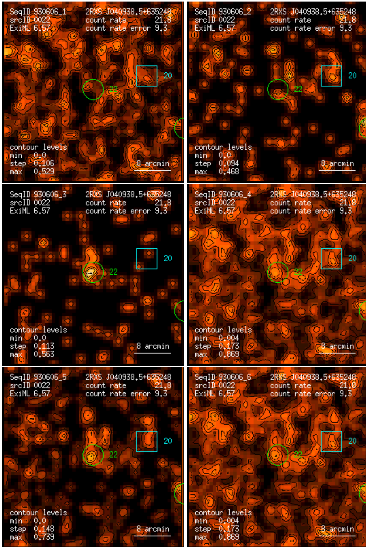
Figure 22: RASS 930606: detection 0022: band rate images, Gaussian filter: (1) PSPC channels 11 – 41, (2) 52 – 90, (3) 91 – 201, (4) 11 – 235, (5) 52 – 201, (6) 11 – 201. Broad band rates in counts/ks. Band rate contour levels in counts/ks/arcmin 2 .
