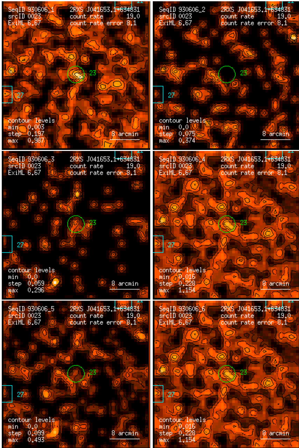
Figure 23: RASS 930606: detection 0023: band rate images, Gaussian filter: (1) PSPC channels 11 – 41, (2) 52 – 90, (3) 91 – 201, (4) 11 – 235, (5) 52 – 201, (6) 11 – 201. Broad band rates in counts/ks. Band rate contour levels in counts/ks/arcmin 2 .
