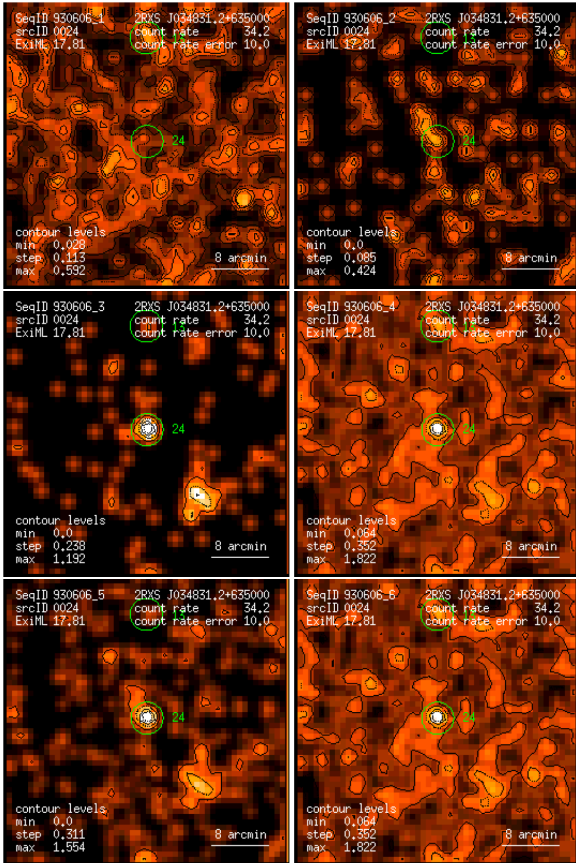
Figure 24: RASS 930606: detection 0024: band rate images, Gaussian filter: (1) PSPC channels 11 – 41, (2) 52 – 90, (3) 91 – 201, (4) 11 – 235, (5) 52 – 201, (6) 11 – 201. Broad band rates in counts/ks. Band rate contour levels in counts/ks/arcmin 2 .
