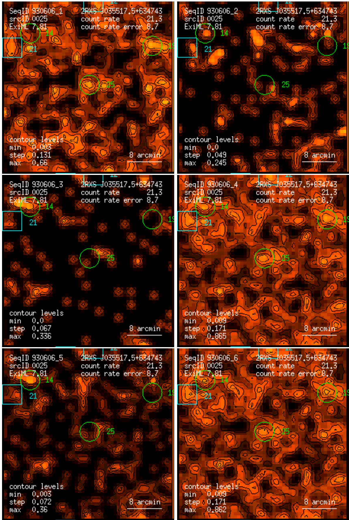
Figure 25: RASS 930606: detection 0025: band rate images, Gaussian filter: (1) PSPC channels 11 – 41, (2) 52 – 90, (3) 91 – 201, (4) 11 – 235, (5) 52 – 201, (6) 11 – 201. Broad band rates in counts/ks. Band rate contour levels in counts/ks/arcmin 2 .
