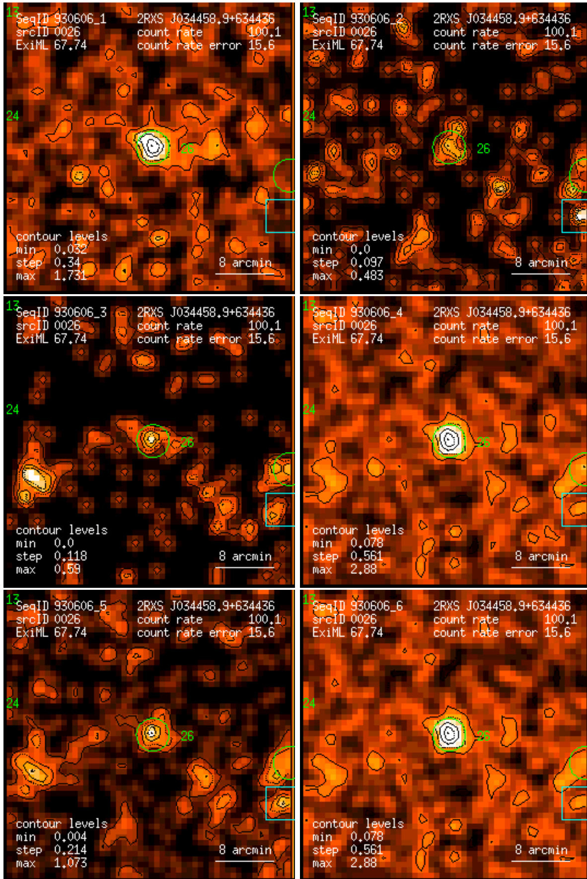
Figure 26: RASS 930606: detection 0026: band rate images, Gaussian filter: (1) PSPC channels 11 – 41, (2) 52 – 90, (3) 91 – 201, (4) 11 – 235, (5) 52 – 201, (6) 11 – 201. Broad band rates in counts/ks. Band rate contour levels in counts/ks/arcmin 2 .
