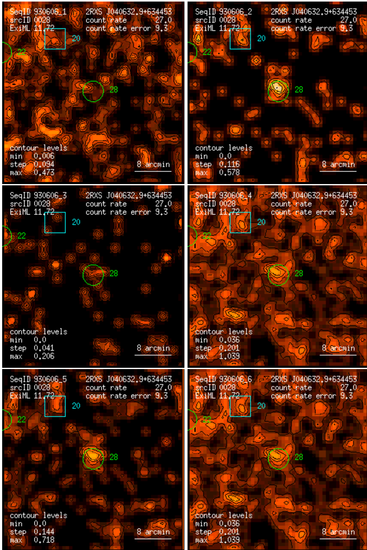
Figure 28: RASS 930606: detection 0028: band rate images, Gaussian filter: (1) PSPC channels 11 – 41, (2) 52 – 90, (3) 91 – 201, (4) 11 – 235, (5) 52 – 201, (6) 11 – 201. Broad band rates in counts/ks. Band rate contour levels in counts/ks/arcmin 2 .
