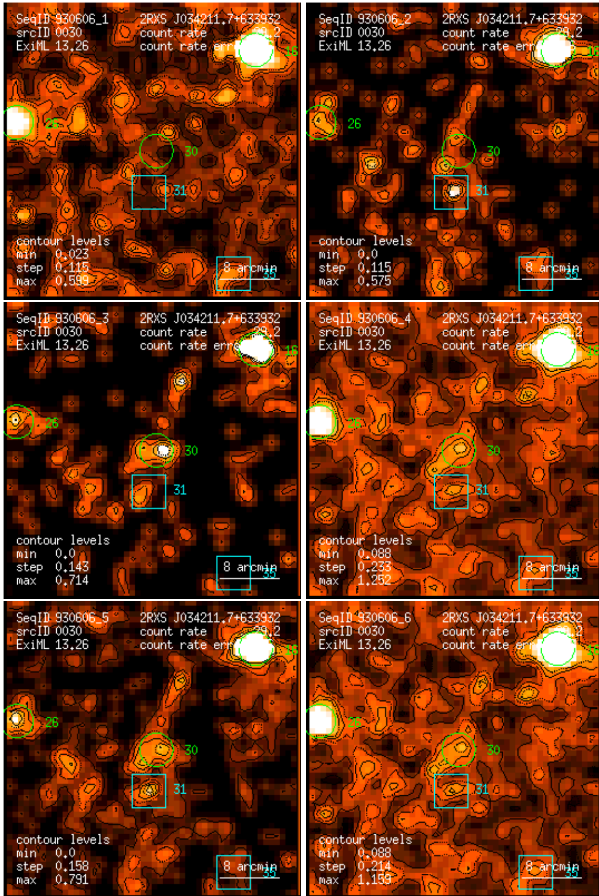
Figure 30: RASS 930606: detection 0030: band rate images, Gaussian filter: (1) PSPC channels 11 – 41, (2) 52 – 90, (3) 91 – 201, (4) 11 – 235, (5) 52 – 201, (6) 11 – 201. Broad band rates in counts/ks. Band rate contour levels in counts/ks/arcmin 2 .
