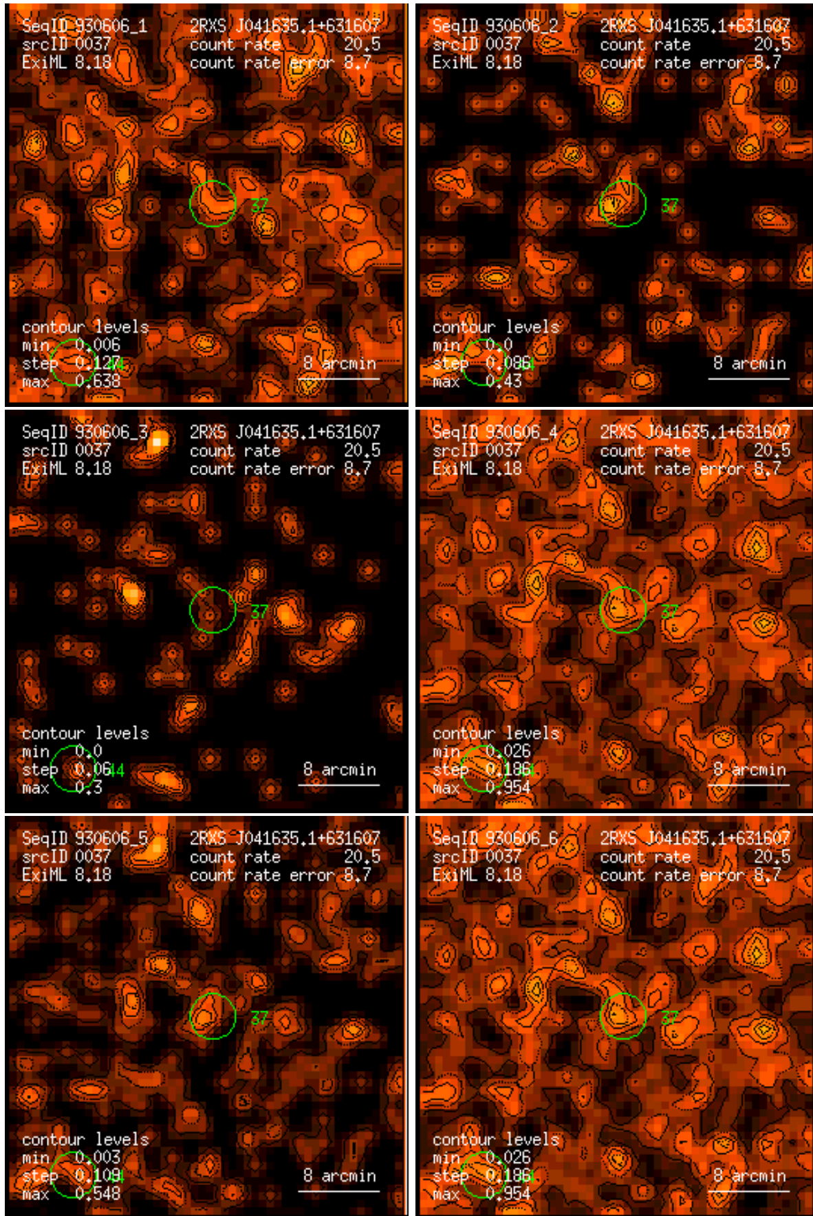
Figure 37: RASS 930606: detection 0037: band rate images, Gaussian filter: (1) PSPC channels 11 – 41, (2) 52 – 90, (3) 91 – 201, (4) 11 – 235, (5) 52 – 201, (6) 11 – 201. Broad band rates in counts/ks. Band rate contour levels in counts/ks/arcmin 2 .
